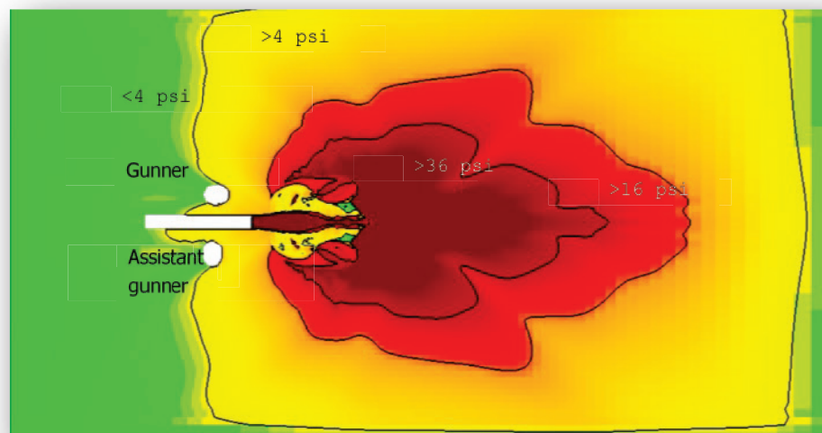
Figure 5.1. Typical Blast Overpressure Map for Shoulder-Fired Heavy Weapons
