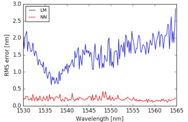
Figure 8. Comparison of wavelength modeling using a linear model (LM, blue curve) and a neural network (NN, red curve).
