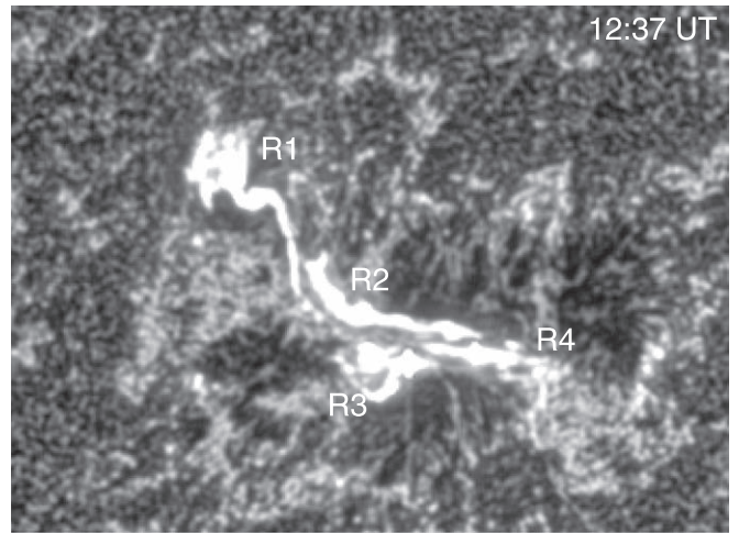
Figure 2. Location of ribbon pairs R1–R2 and R3–R4 in SDO / AIA 1600 Å image at 12:37 UT during flare FL1.
