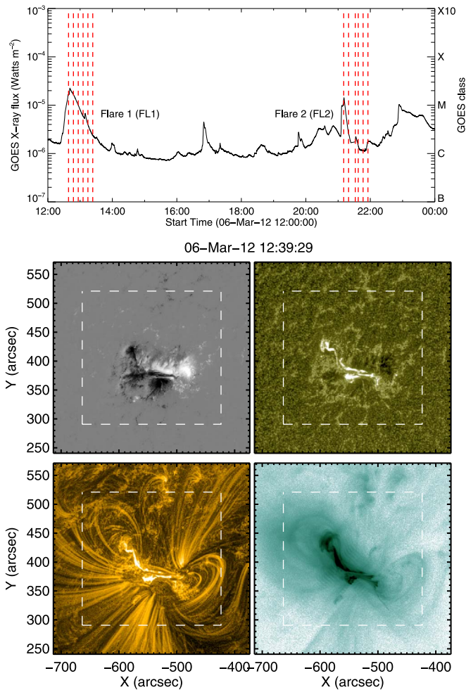
Figure 1. Top panel: GOES soft X-ray curve from 12:00 UT on 2012 March 6 to 00:00 on March 7 with Hinode / EIS raster times indicated by the dashed red lines. Flare 1 (M2.2) peaked at \sim 12:37 UT and Flare 2 (M1.4) peaked at \sim 21:12 UT. Bottom panel: clockwise from upper left: SDO / HMI line-of-sight (LOS) magnetogram, SDO / AIA 1600 Å, 94 Å, and 171 Å maps of AR 11429 at 12:39 on 2012 March 6 overlaid with the Hinode / EIS field of view (dashed white box). The animation of the bottom panels begins at 11:44:44 and ends at 22:29:44. Its duration is 28 s. Note that the cadence of the animation is 45 s for the flare periods but is 5 minutes from 14:00 UT to 20:15 UT.
