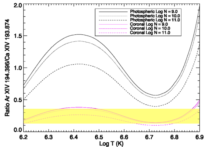
Figure 7. Intensity ratios of Ar XIV and Ca XIV contribution functions vs. electron temperature for electron densities of \log_{10} N = 9.0, 10.0, 11.0 . Shaded box shows the range of the Ar XIV/Ca XIV ratio in the temperature range of [6.2, 6.8] for electron density of \log_{10} N = 10.0 and coronal abundances as given in Section 3.1. The ratio is quite narrow for a wide temperature range but exceeds 0.50 for temperatures above \log_{10} T = 6.9 K.
