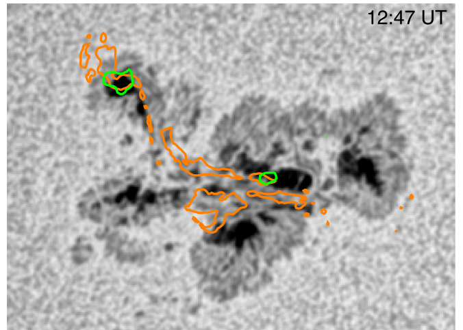
Figure 6. SDO /HMI Continuum at 12:47 UT overlaid with contours of IFIP (green) and flare ribbons (orange). The contours overlap at the umbrae associated with ribbon pairs R1–R2. IFIP contours are from the Hinode /EIS Ar XIV/Ca XIV intensity ratio map at 12:47 UT in Figure 4. Flare ribbon contours are from the SDO /AIA 1600 image Å at 12:37 UT in Figure 2 adjusted for solar rotation.
