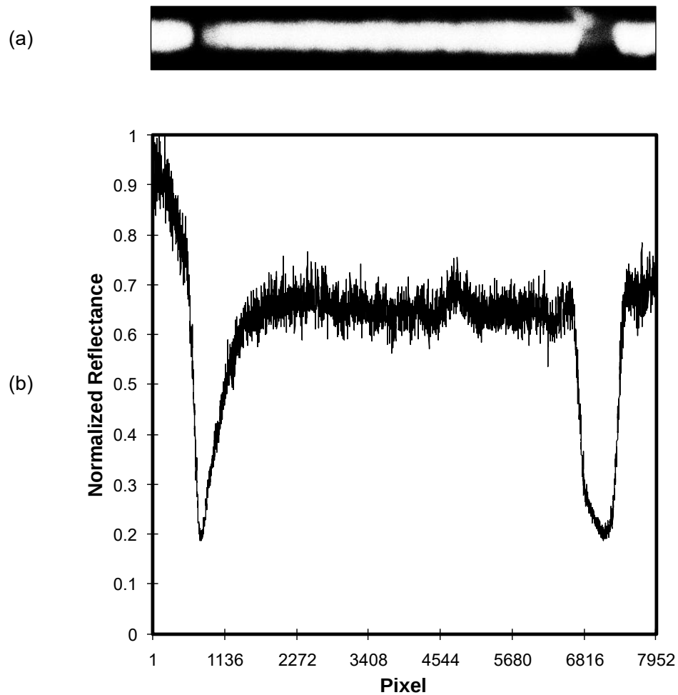
Figure 9. (a) SPR reflectivity pattern of air and water and (b) its corresponding normalized reflectivity averaged along the vertical direction.
