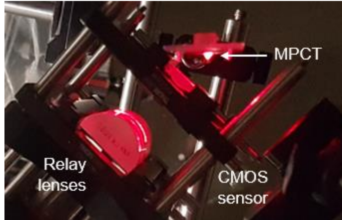
Figure 16. Experimental demonstration of the SPR sensing using the MPCTC.
