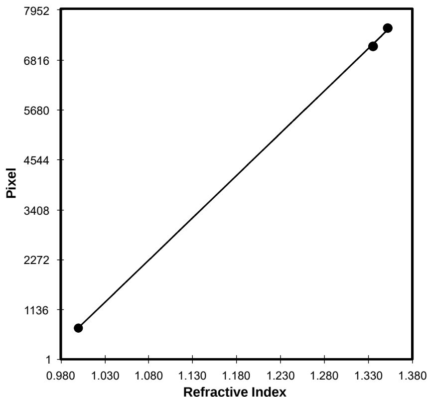
Figure 13. Detected SPR positions as a function of the refractive index of the test samples.
