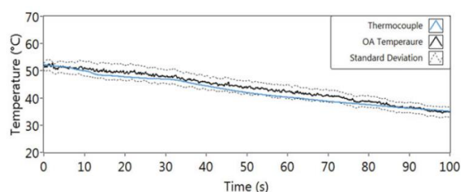
Fig. 2. The temperature, measured by a thermocouple (reference temperature, blue line), and the simultaneously obtained T_{OA} (black solid line, standard deviation with black dash lines) of the culture medium during cooling from about 52°C to 35°C. {Miura, 2019 #15}
