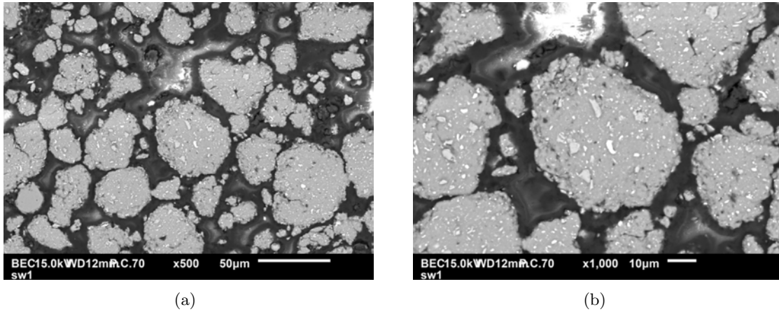
Figure 9. Sectioned \text{Al-Si10-Mg} + 10 \text{ wt\% TiB}_2 particles after 240 min of mechanical alloying: (a) 500 \times magnification; (b) 1000 \times magnification. (Mill speed=450 rpm, BPR=10, PCA: stearic acid at 2 wt%.)
