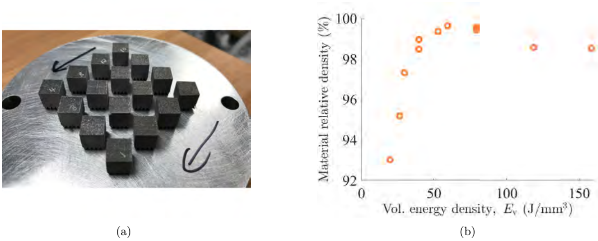
Figure 18. Laser consolidation of bulk samples of Al-Si10-Mg: (a) 1\text{ cm}^3 density cubes built with P=190\text{--}380\text{ W} and v=500\text{--}2000\text{ mm/s} ; (b) The relative density of the samples peaks at volumetric energy densities in the range E_v=52.8\text{--}79.2\text{ J/mm}^3 .
