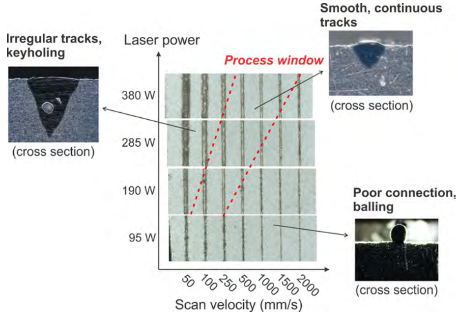
Figure 17. Process window for plain Al-Si10-Mg powder determined from single track melting experiments (75 \mu\text{m} powder layer spread on Al-12Si substrate).
