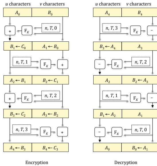
Figure 15. FF1 Feistel Structure
