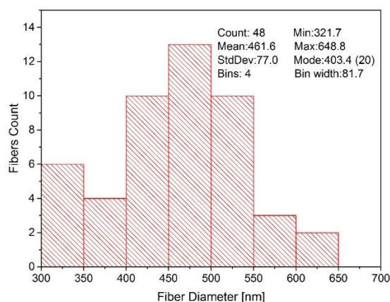
Figure 21: Sub-group A7. (a) SEM observation. (b) Fibres size distribution
