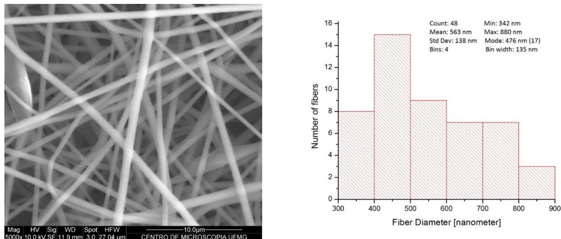
Figure 4: HRSEM Observation
