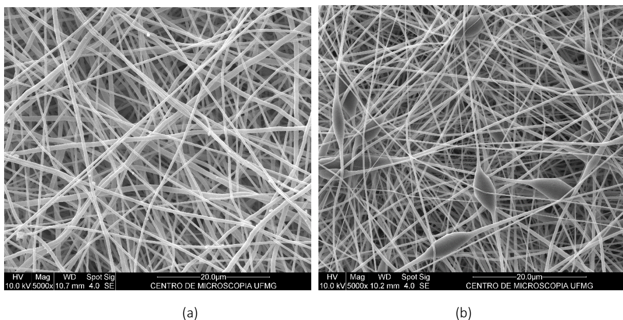
Figure 27: Nanomembranes. (a) PVDF nanomembrane; (b) PVDF-HFP nanomembrane near-bead free
