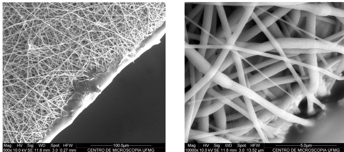
Figure 5: HRSEM – Interface substrate/nanomembrane
