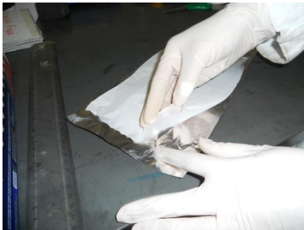
Figure 35. Nanomembrane prepared by electrospinning. (a) Removing from substrate; (b) stretching.
