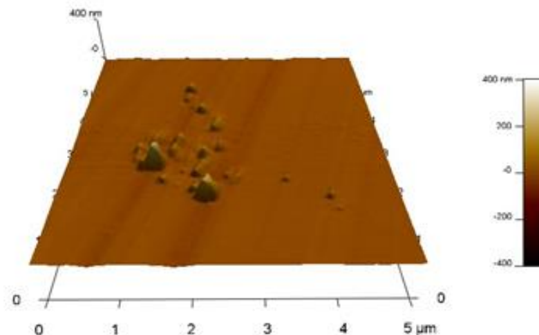
Figure 3: AFM observation
