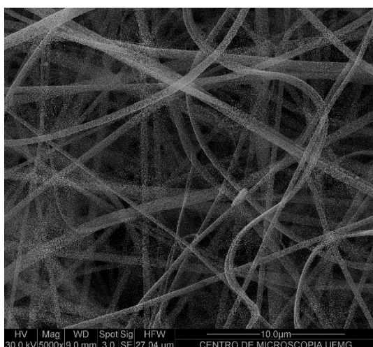
Figure 21: Sub-group A7. (a) SEM observation. (b) Fibres size distribution
