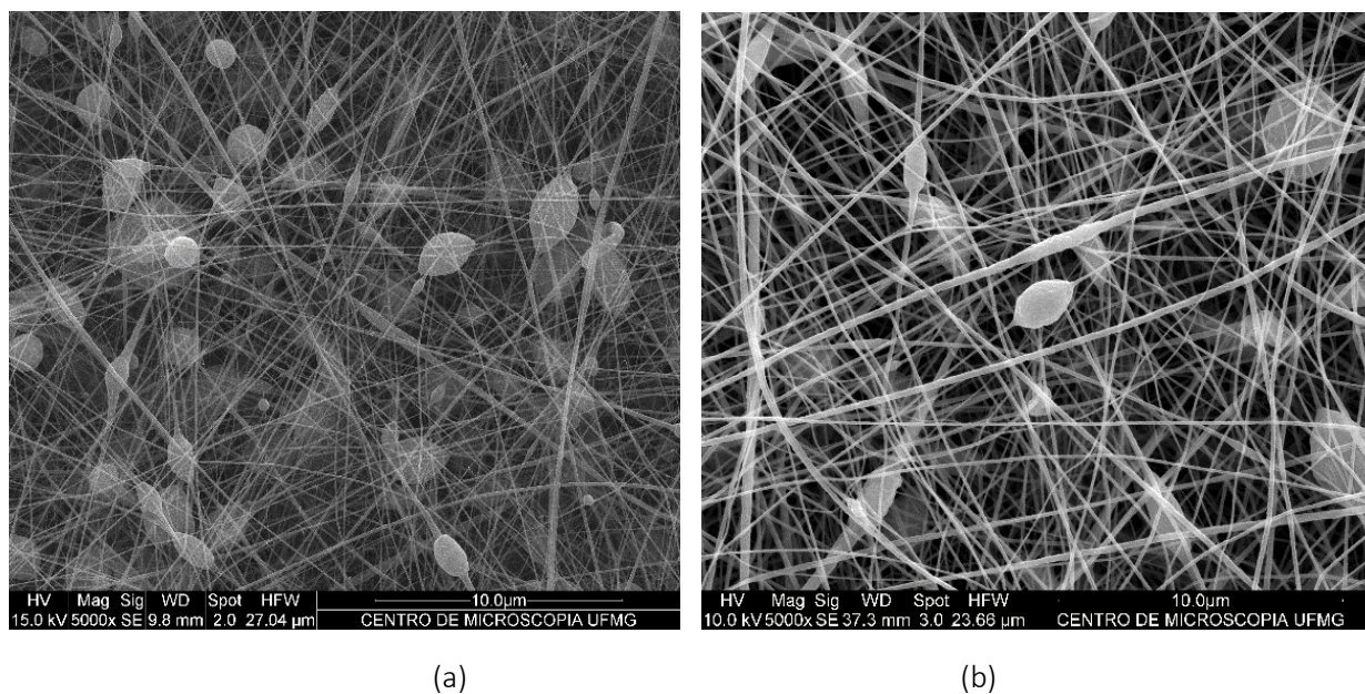
Figure 26: Nanomembranes with beads. (a) PVDF nanomembrane; (b) PVDF-HFP nanomembrane
