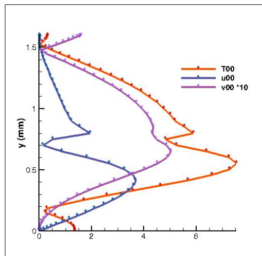
Figure 4: Mean flow corrections(MFC)
