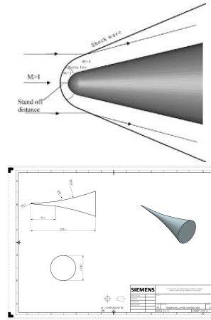
Figure 2: Mean flow configurations
