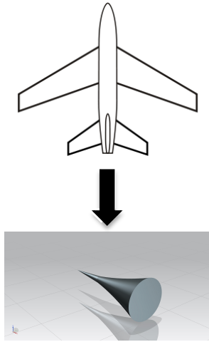
Figure 1: PSE code boundary layer profile change
