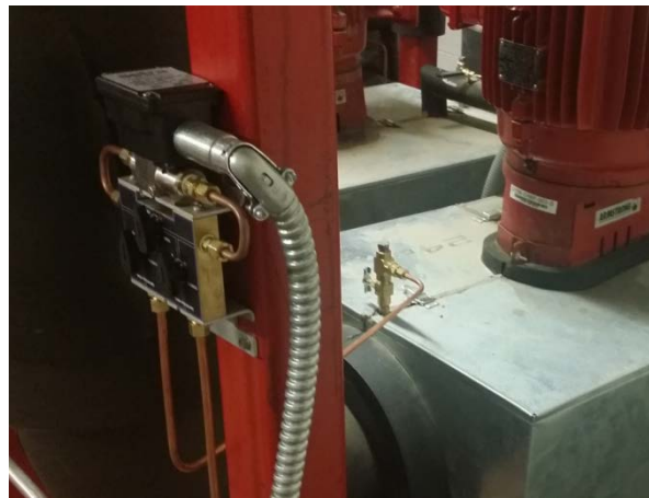
Figure 5.12. Permanent Differential Pressure Transducer Installation for Virtual Pump Flow Meters.
