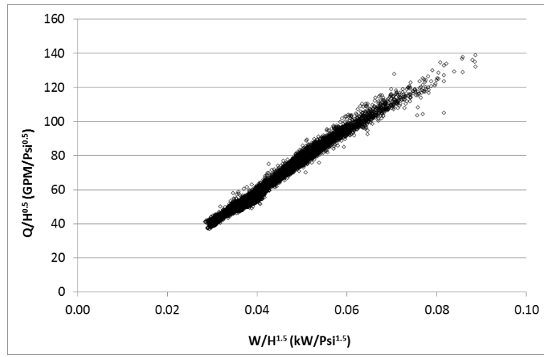
Figure 6.2. Calibrated Pump H/Q^{0.5} versus Ws/H^{1.5} Curve.
