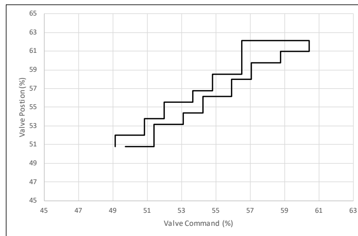
Figure 6.11. Valve Dynamic Behavior Study for Determination of Valve Hysteresis and Stiction.
