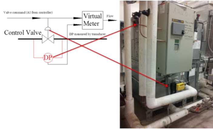
Figure 2.2. Virtual Valve Flow Meter.
