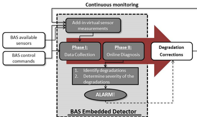
Figure E.1 Flow Chart of the Embedded PDD.
