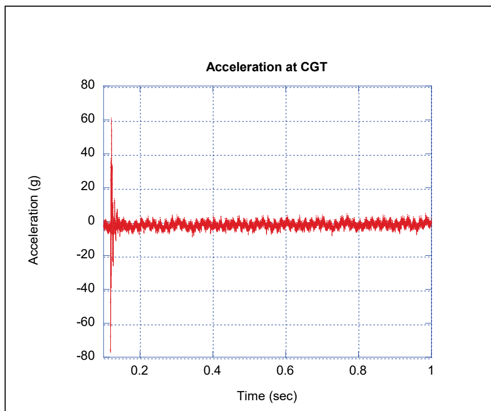
Figure 4. Induced acceleration response at CGT attachment location.
