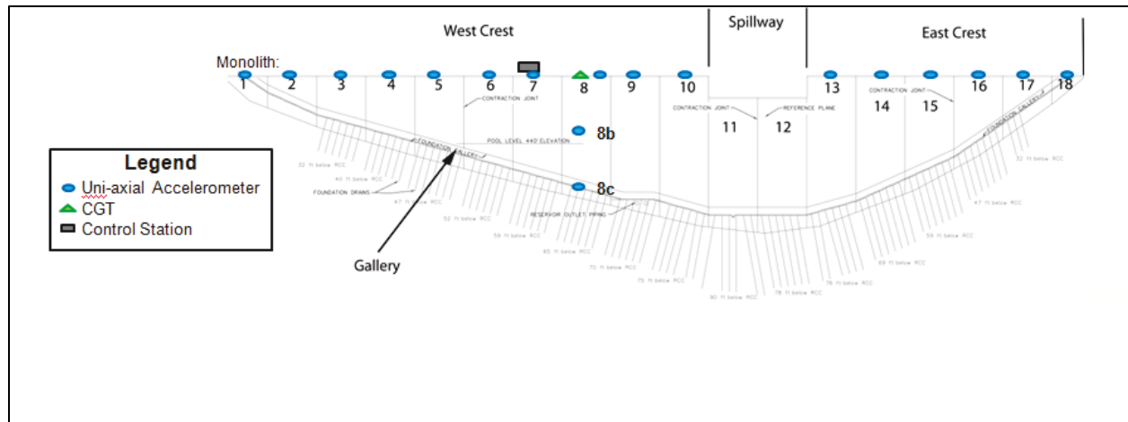
Figure 5. Measurement layout.
