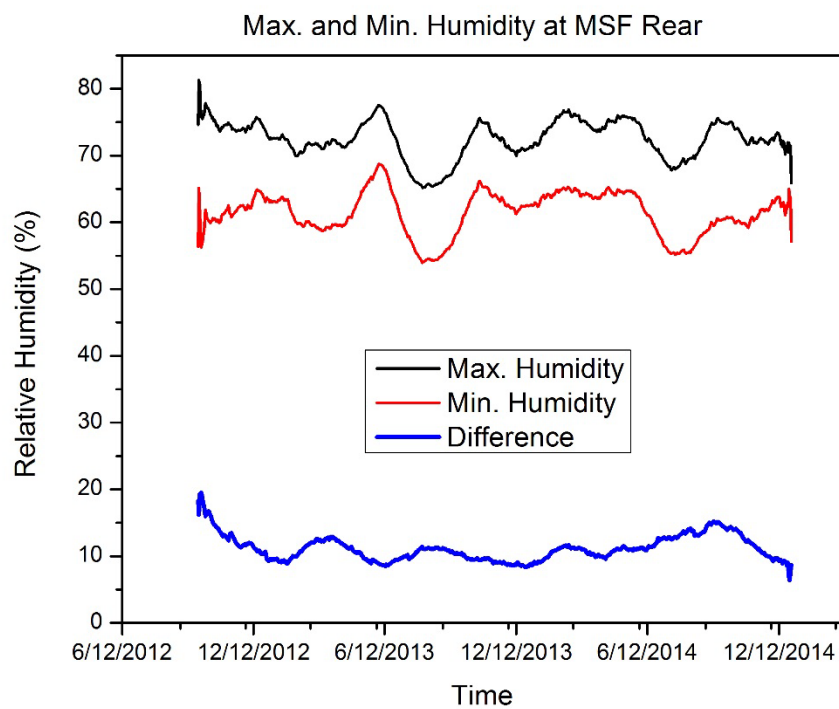
Figure 12. Maximum and minimum humidity at the rear of the MSF.
