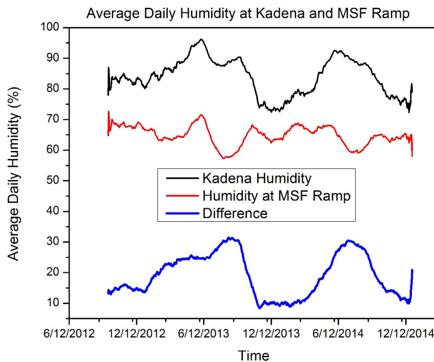
Figure 9. Average daily outdoor humidity at Kadena and inside the MSF at front (ramp).
