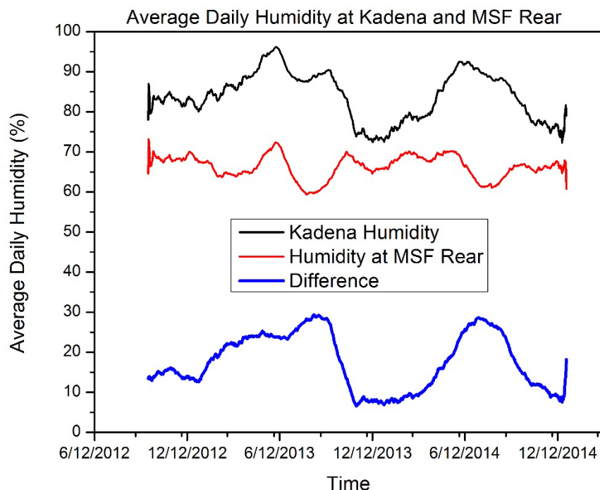
Figure 10. Average daily outdoor humidity at Kadena and inside the MSF at the rear.
