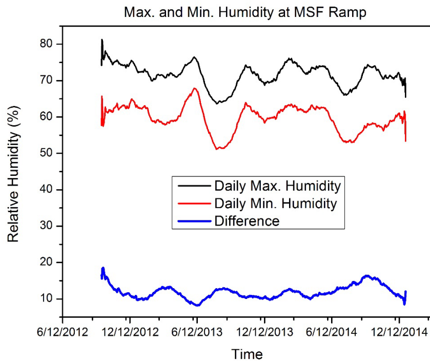
Figure 11. Maximum and minimum humidity at the front of the MSF (ramp).
