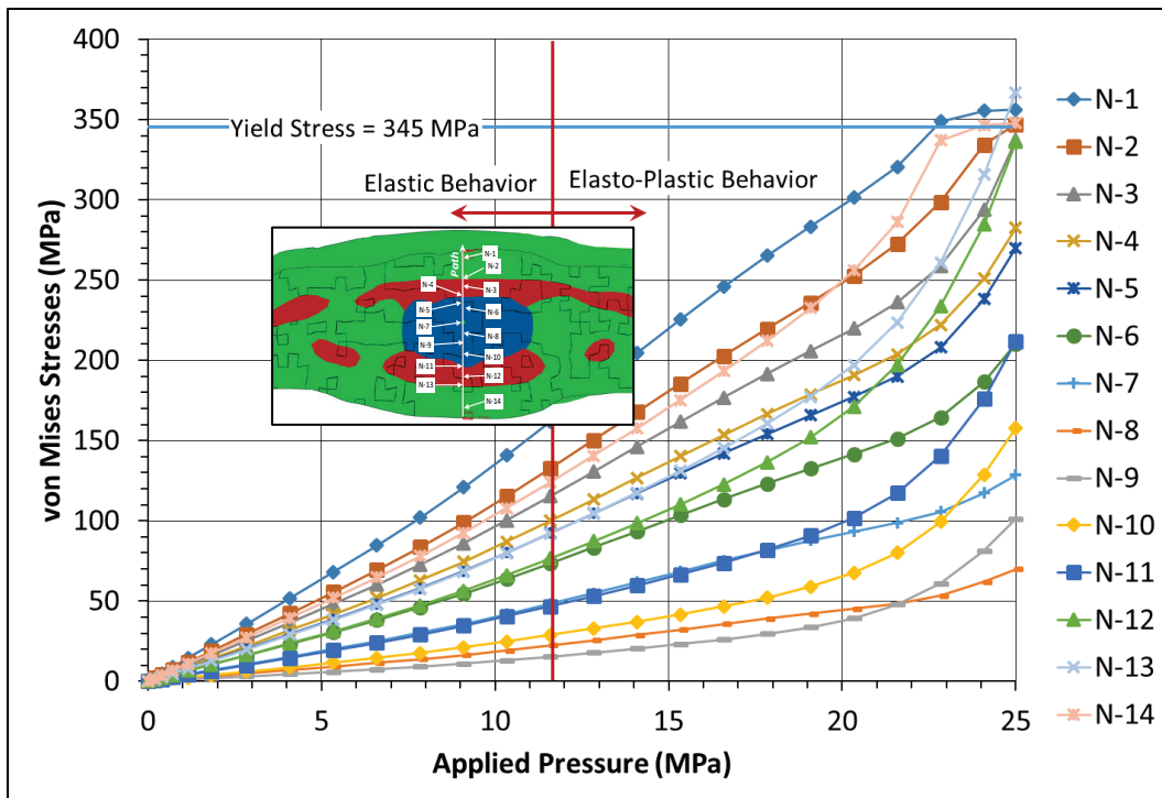
Figure 28. Variation of von Mises stresses at selected nodes with applied pressure at the center of the rostrum for the second-order-reduced integration model. (Reference in Figure 27).
