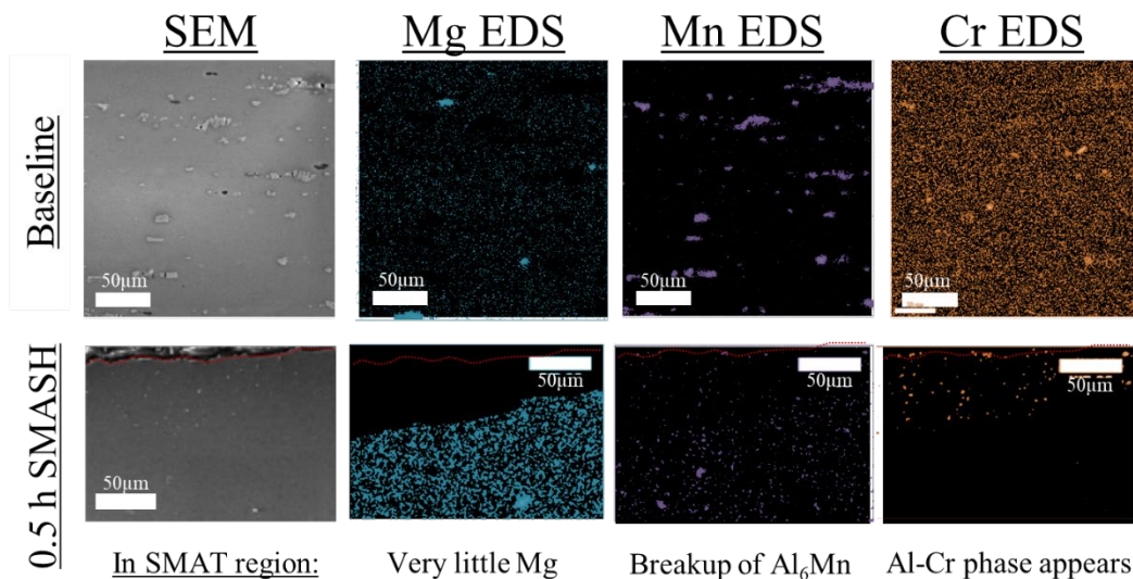
Fig. 10 (top row) SEM images and EDS maps of unsensitized baseline AA5083 and (bottom row) SMASH for 0.5 h, steel media. Treated surface is indicated by red dashed line.
