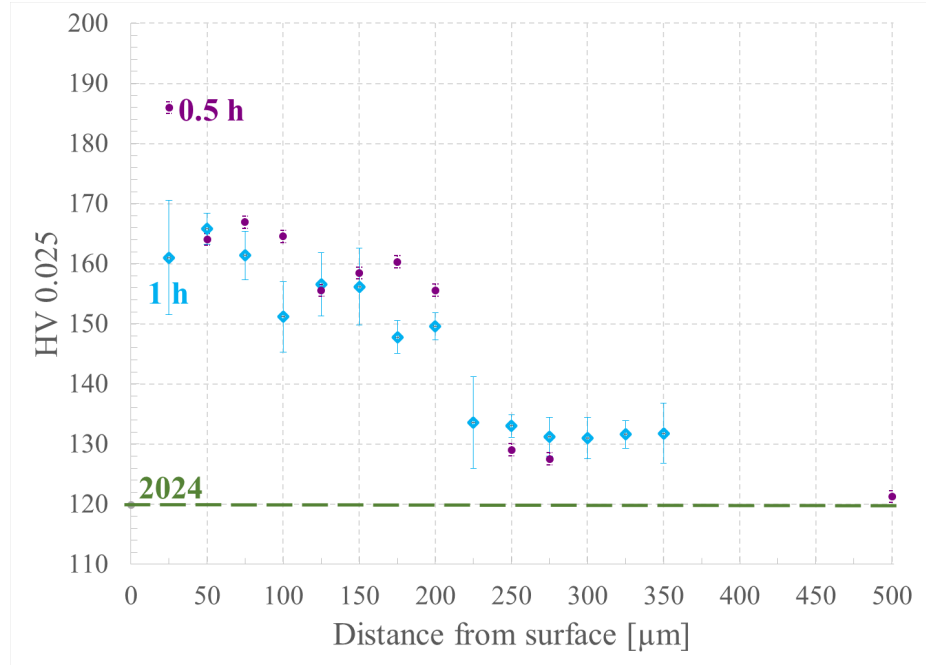
Fig. 5 Microhardness of the AA2024 SMASH treated with steel media for 0.5 h (purple circles) and 1 h (aqua diamonds) as a function of depth into the substrate. Baseline AA2024 hardness is indicated by green dashed line.
