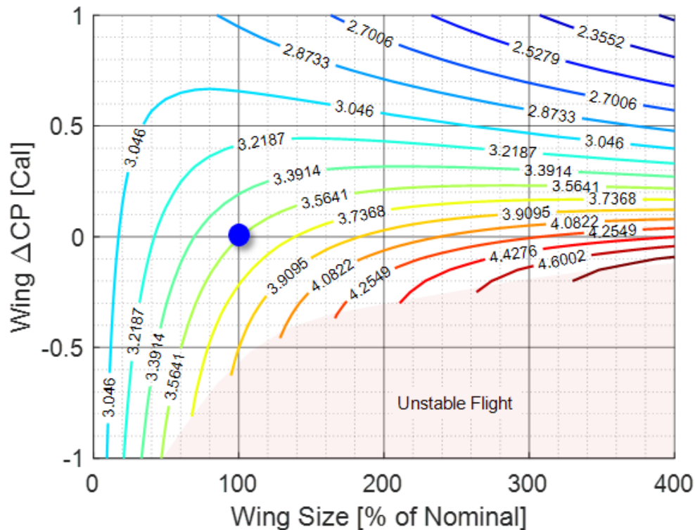
Fig. 14 Lift-to-drag ratio at steady-state trim angle of attack, plotted as a function of wing size and center of pressure at Mach 0.5. The nominal wing design is shown with a blue dot.
