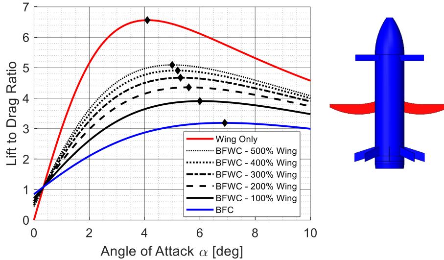
Fig. 8 Lift-to-drag ratio for the BFC, the wing alone, and the BFWC for several wing sizes at Mach 0.5. The optimal angles of attack corresponding to the highest lift-to-drag ratios for each configuration are marked with diamonds.
