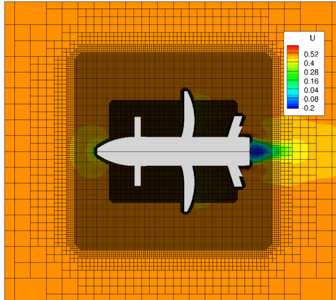
Fig. 3 Contour of simulated non-dimensional streamwise velocity superimposed with the computational domain (Cart3D)
