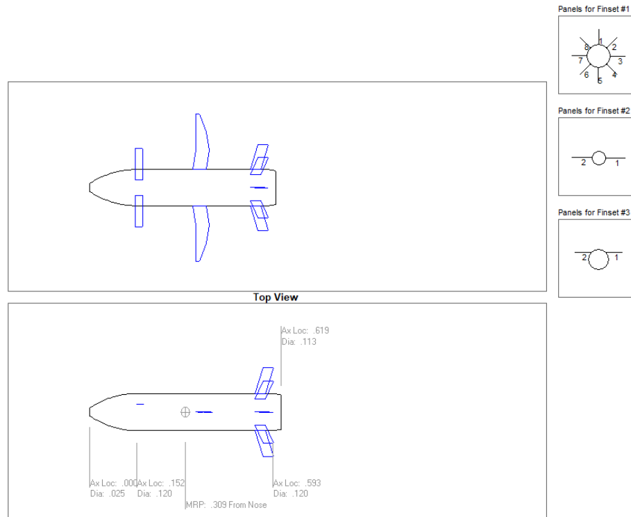
Fig. 2 Geometry sketch of projectile concept modeled in MissileLab and executed in Missile DATCOM
