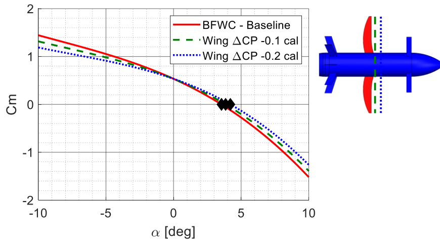
Fig. 13 BFWC static pitching moment at Mach 0.5 for nominally sized wings acting on the body at different CPs, with +5^\circ canard deflection. Steady state trim angles of attack of 3.5^\circ , 3.9^\circ , and 4.2^\circ are indicated with diamonds.
