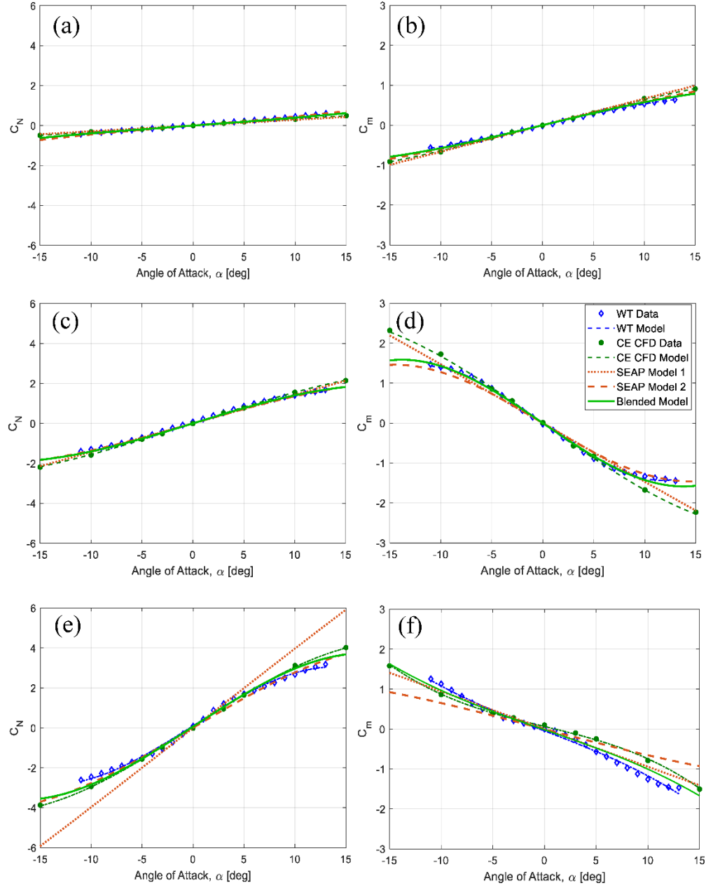
Fig. 5 Normal force coefficient (a, c, e) and pitching moment coefficient (b, d, f) of B (a–b), BF (c–d), and BFWC (e–f) configurations at Mach 0.2 from WT only, CE CFD only, SEAP only, and blended (SEAP, CE CFD, and WT) data
