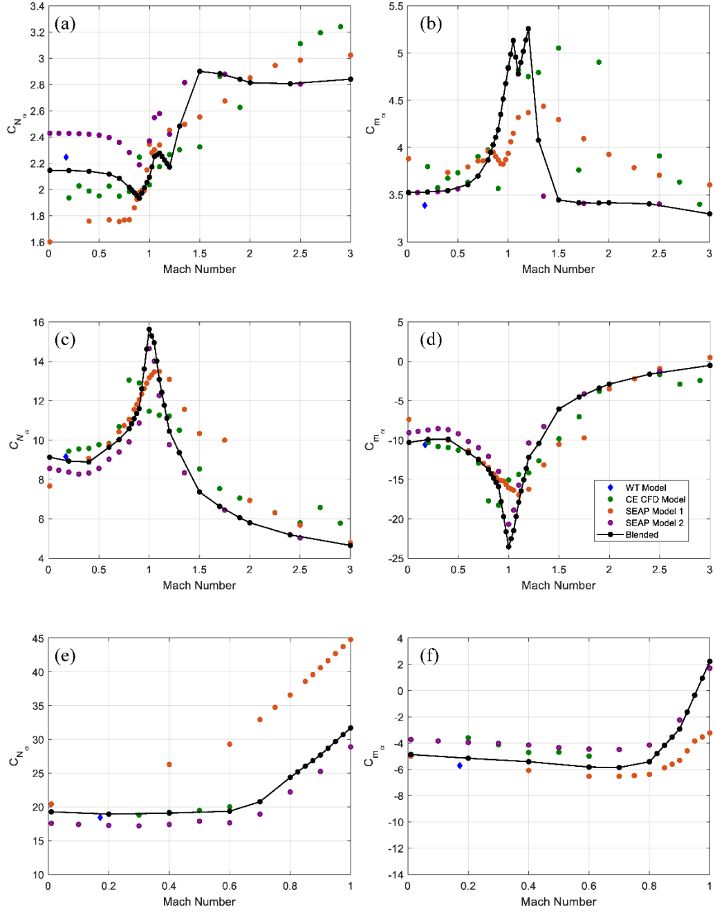
Fig. 7 First-order coefficient of static normal force and static pitching moment for BF and BFWC configurations from SEAP, CE CFD, WT only, and blended (SEAP, CE CFD, and WT) data across Mach number
