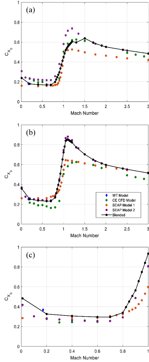
Fig. 6 Zeroth-order coefficient of axial force for B (a), BF (b), and BFWC (c) configurations from SEAP, CE CFD, WT only, and blended (SEAP, CE CFD, and WT) data across Mach number.
