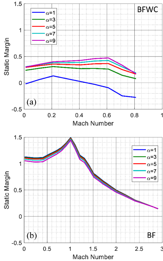
Fig. 9 Static margin of BF and BFWC configurations for varying \alpha
