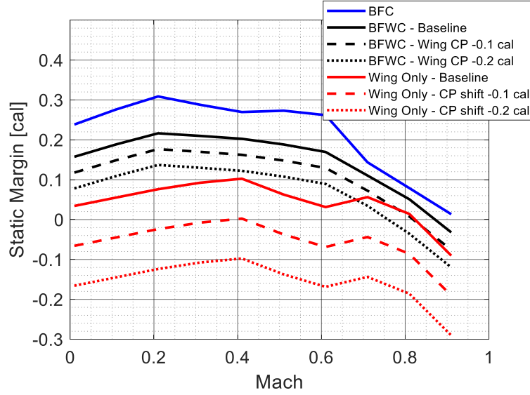
Fig. 11 Effect of shifting wing CP on wing static margin and static margin of BFWC. Shifting the wing CP toward the nose decreases the total stability.
