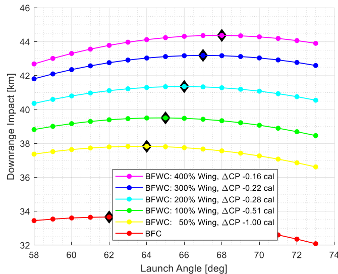
Fig. 15 Range as a function of launch angle for several configurations. Optimal launch angles for each are highlighted with a diamond.
