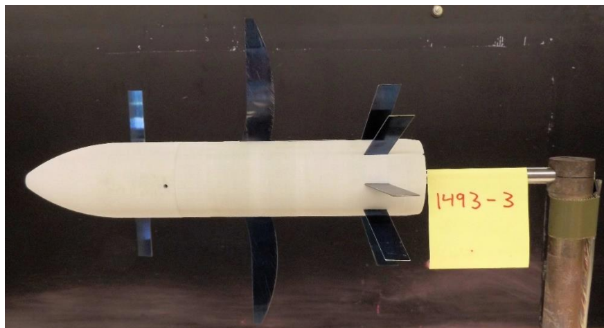
Fig. 4 Instrumented model mounted in WT facility test section
