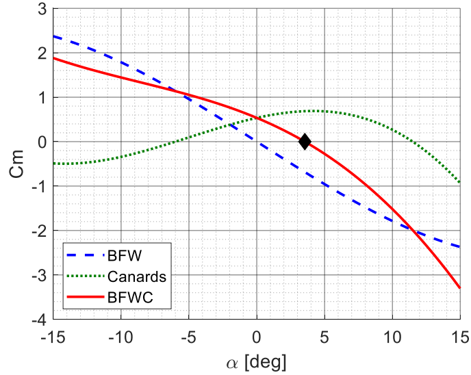
Fig. 12 Static pitching moment contributions from the BFW, from canards alone with +5^\circ deflection, and the combined BFWC for Mach 0.5. The steady-state trim angle of attack of 3.5^\circ is found where the total static pitching moment is zero, as indicated with a diamond.
