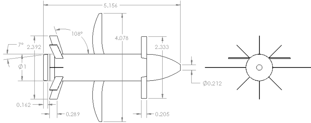
Fig. 1 Projectile concept used in this analysis, showing the nominal wing size and location. Dimensions are given in calibers.
