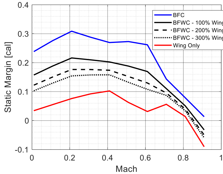
Fig. 10 Static margin at \alpha=3^\circ across Mach for the BFC, for the wing alone, and for the BFWC. Increasing the wing effect decreases the stability.
