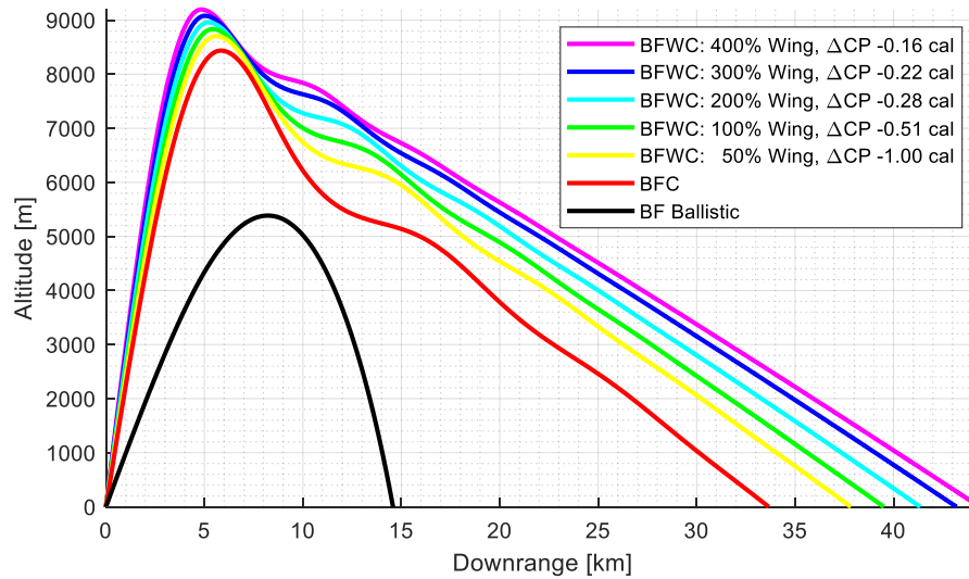
Fig. 16 Trajectories for configurations with the optimized wing designs described in Table 7
