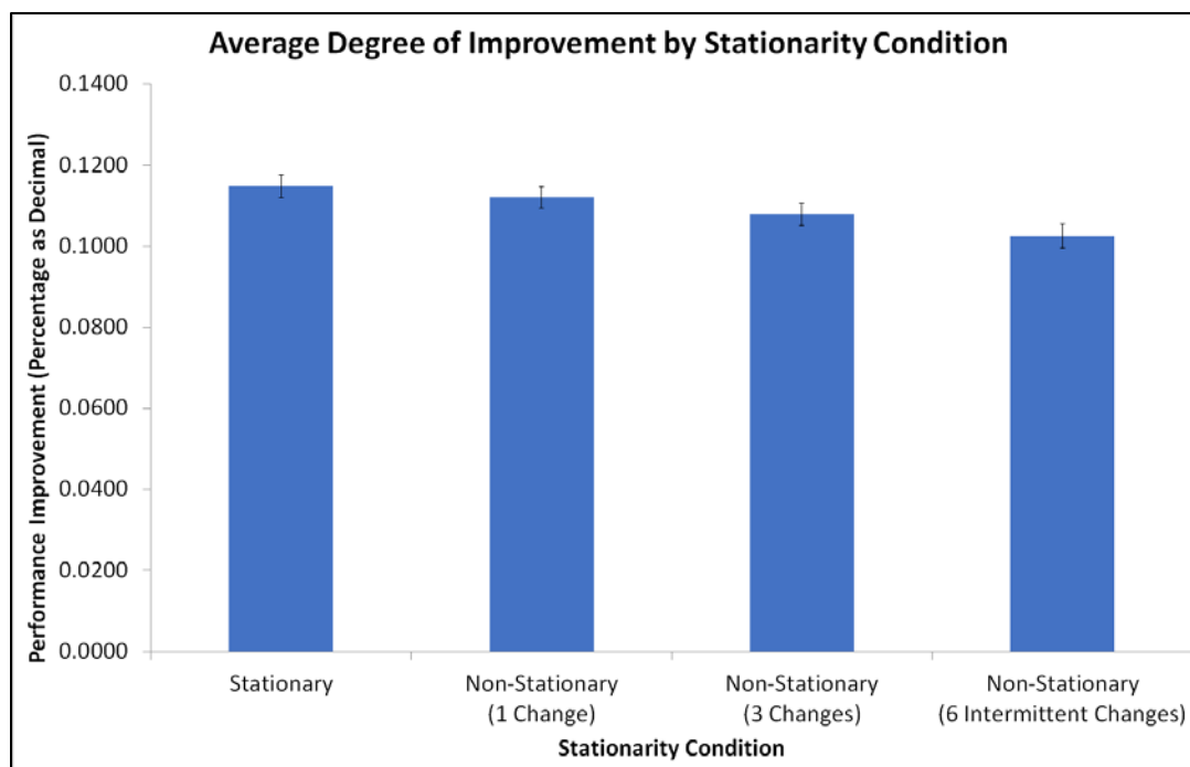
Figure 9: Mean performance improvement for Stationary vs each Nonstationary condition
