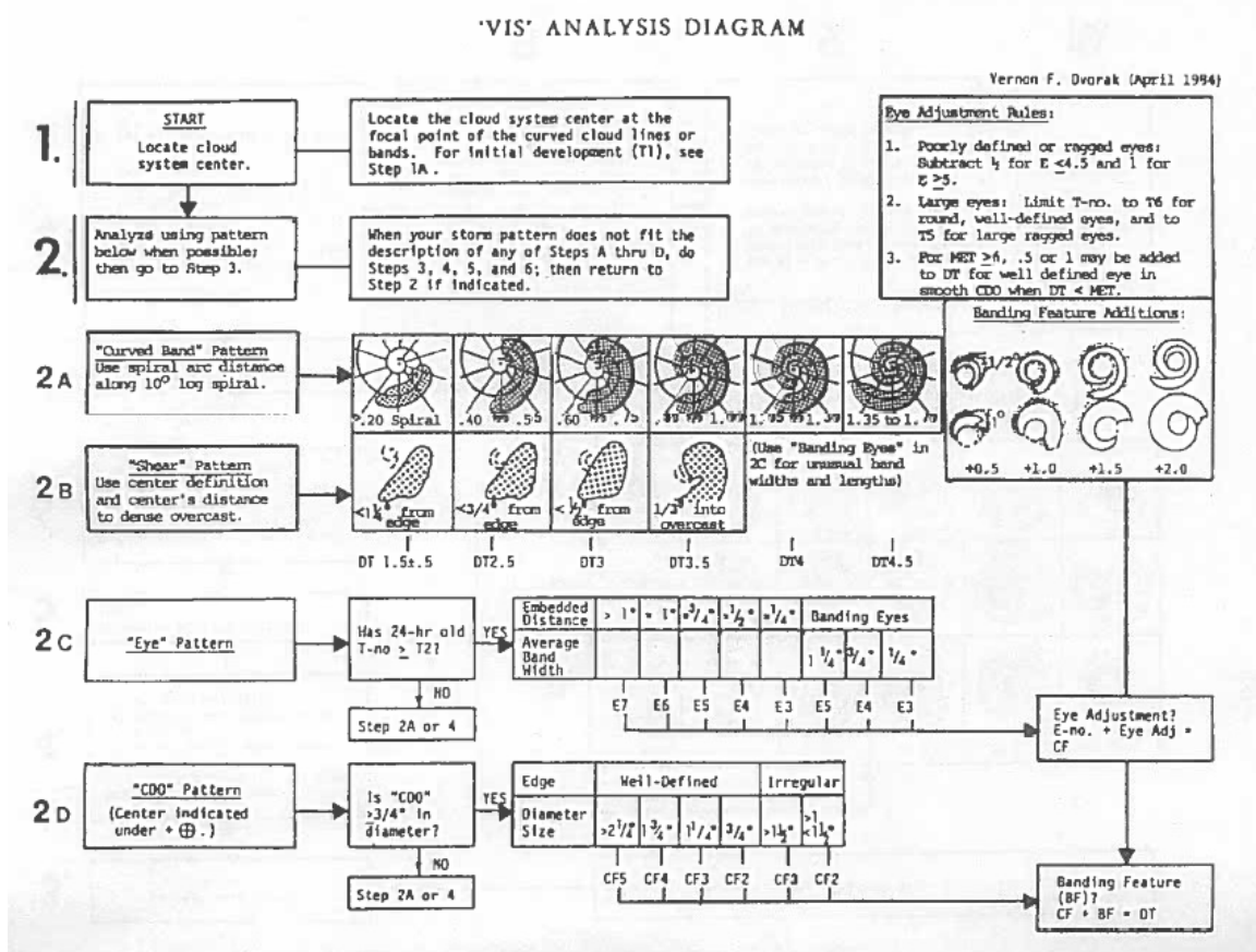
Figure 33. Part 1 of the detailed flow chart to determine intensity using visible imagery (Dvorak, 1984).
