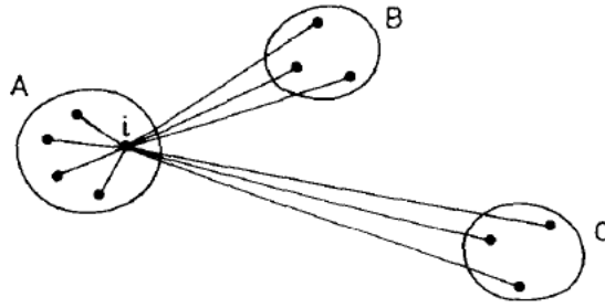
Figure 9. An illustration of the components used to compute s(i) in Equation 1 from Rousseeuw (1987). Used with permission.
