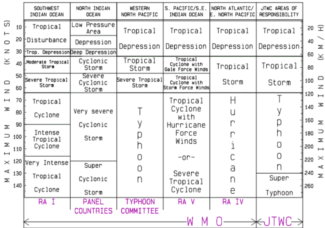
Figure 2. Nomenclature of TCs from World Meteorological Organization (2017). The JTWC nomenclature listed is specific to the Western North Pacific only.
