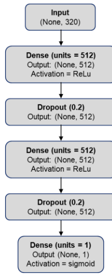
Figure 22: Fully Connected Artificial Neural Network Architecture Diagram
