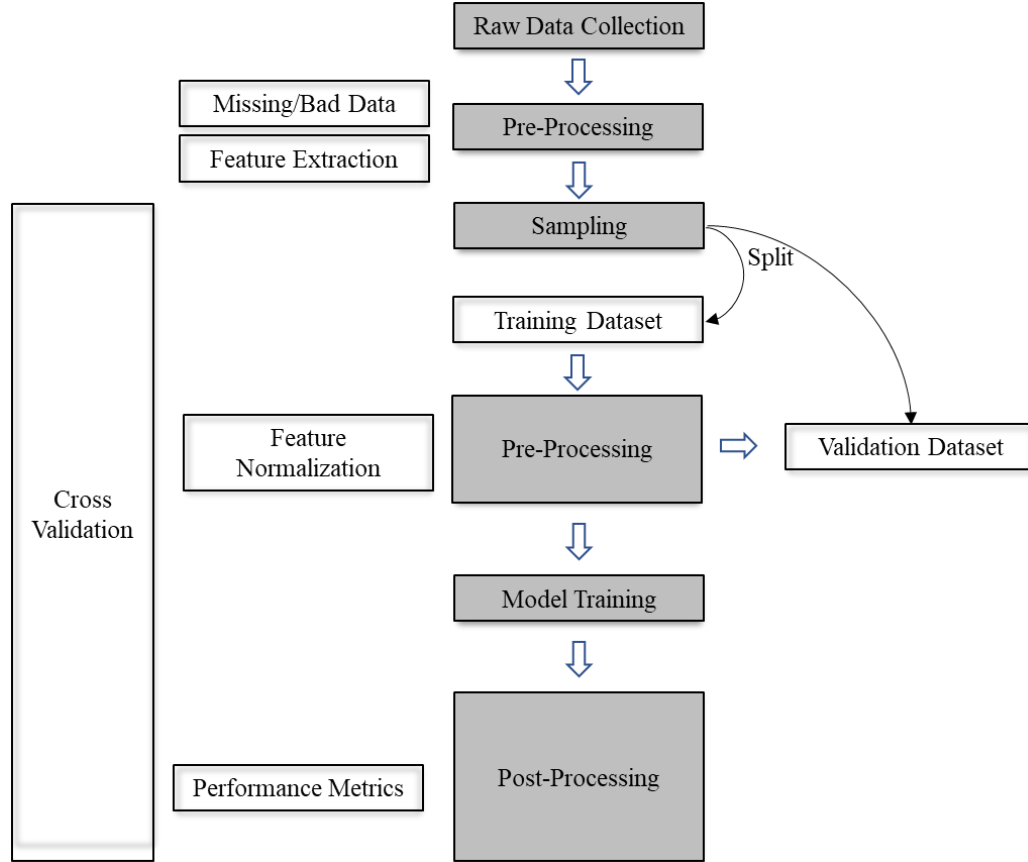
Figure 20: Machine Learning Pipeline
