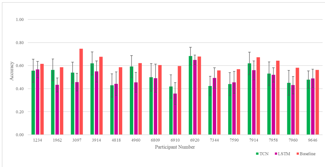
Figure 45: Time Series Information Selection Model Accuracy
