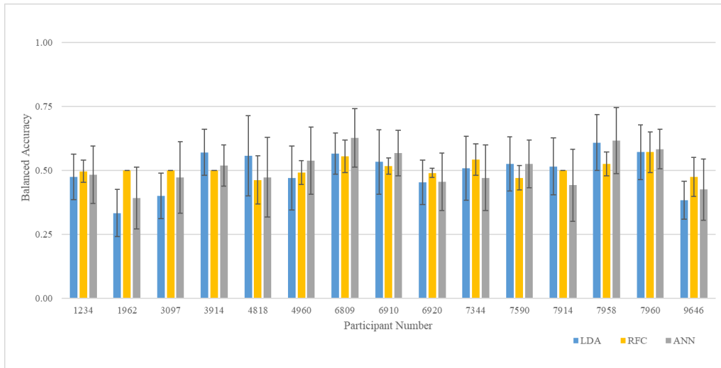
Figure 52: Frequency Information Selection Model Balanced Accuracy
