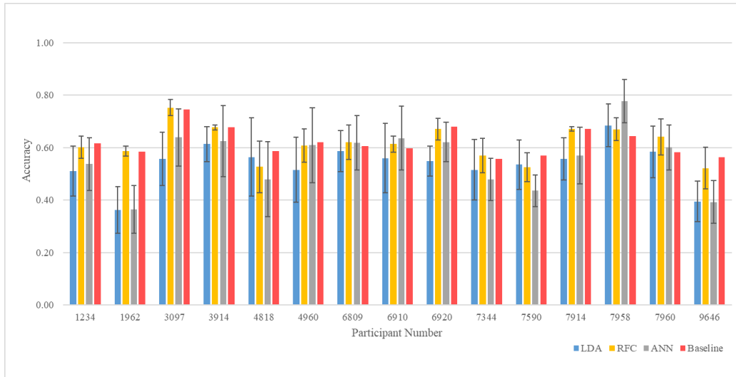
Figure 51: Frequency Information Selection Model Accuracy
