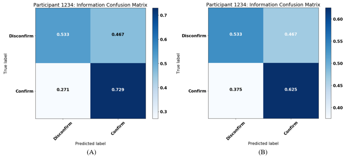
Figure 47: Confusion Matrices (A) TCN, (B) LSTM
