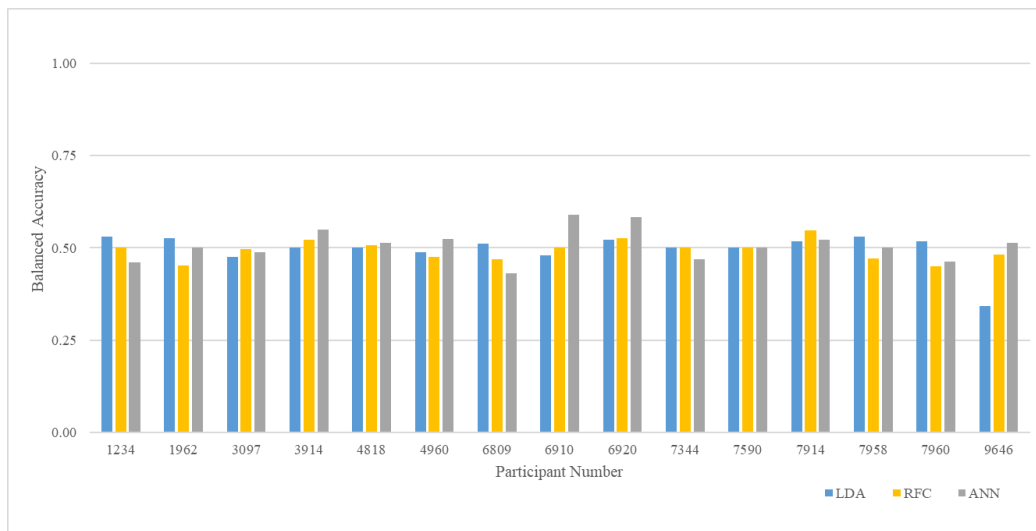
Figure 59: Cross-Participant Model Balanced Accuracy
