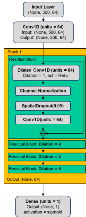
Figure 23: Temporal Convolutional Network architecture diagram.
