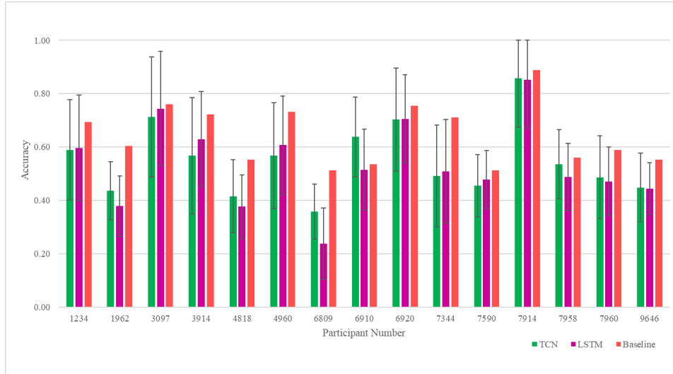
Figure 36: Time Series Signal per Task Model Accuracy
