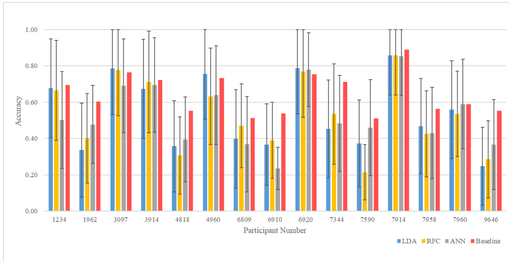
Figure 40: Frequency Features per Task Model Accuracy
