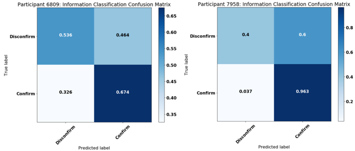
Figure 53: ANN Confusion Matrices
