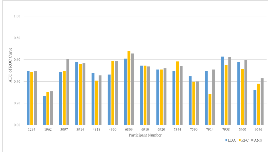
Figure 54: Frequency Information Selection Model AUROC
