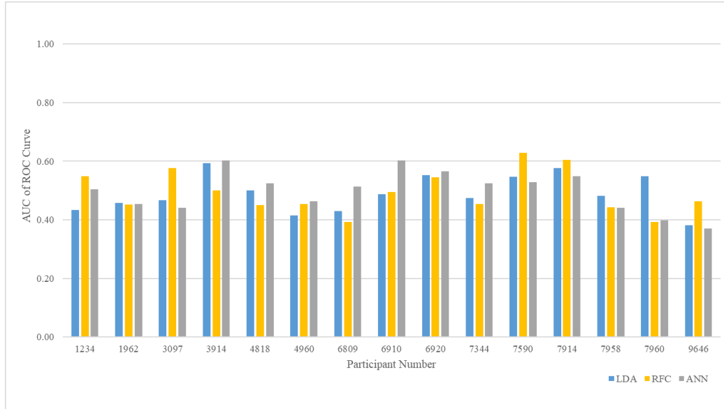
Figure 60: Cross-Participant Model AUROC
