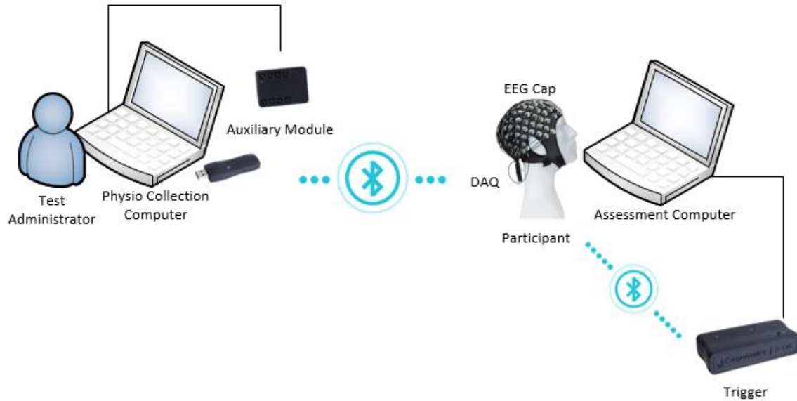
Figure 11: Two Computer Physiological Measurement Collection Set-up
