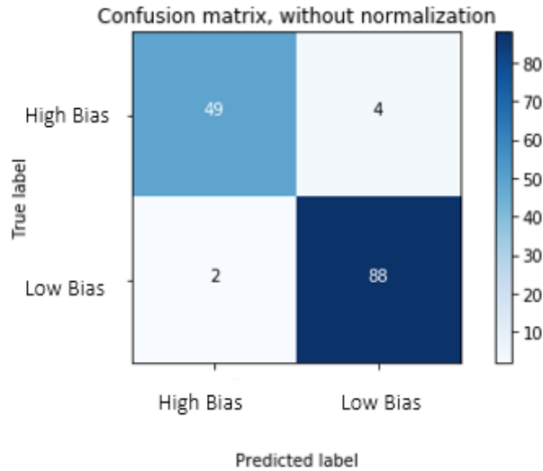
Figure 25: Notional Confusion Matrix for Model Performance on Bias Detection
