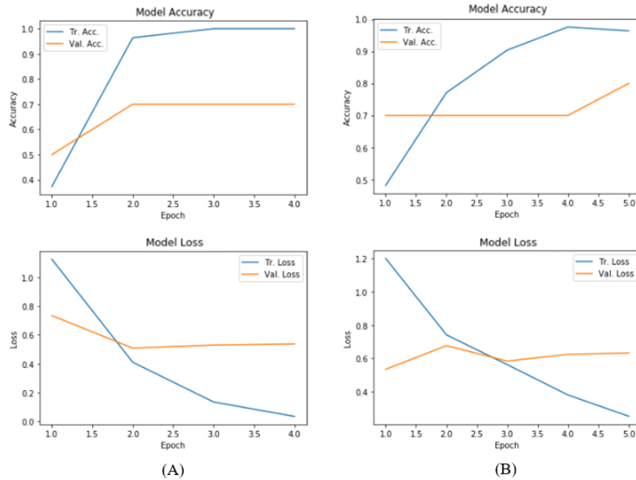
Figure 44: (A) TCN Training Curves (B) LSTM Training Curves
