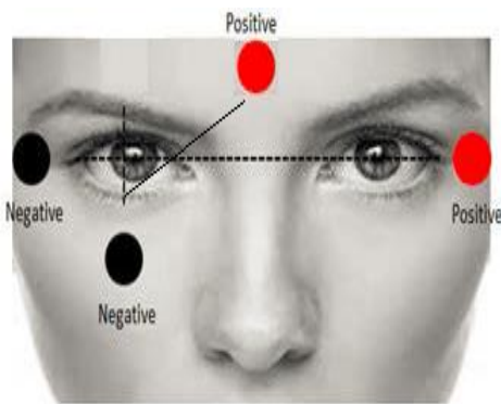
Figure 13: Vertical and Horizontal Electrooculography Node Locations
