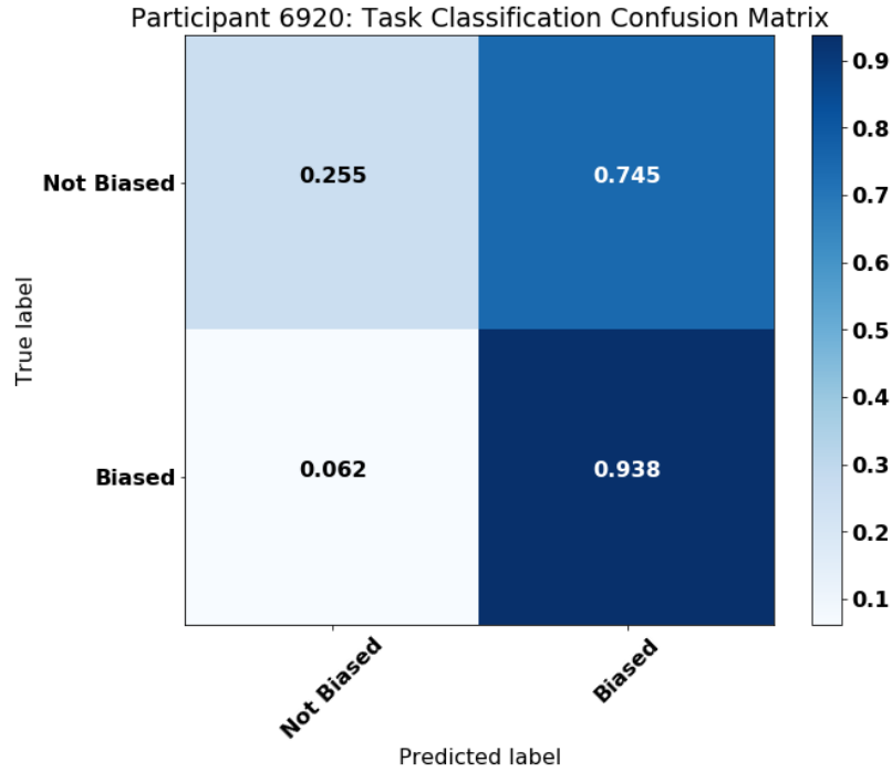
Figure 43: ANN Task Frequency Confusion Matrix
