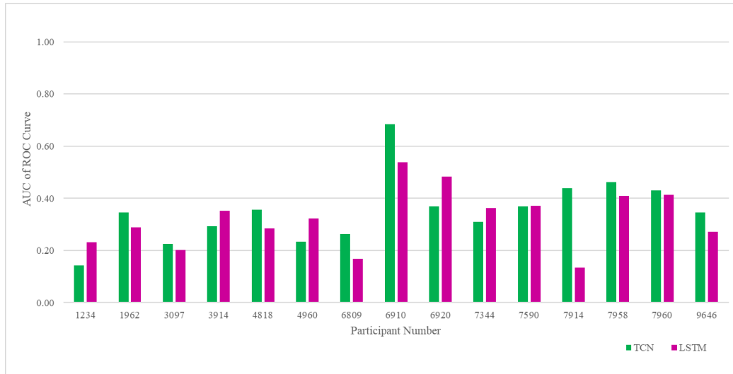
Figure 38: Time Series Signal per Task Model AUROC
