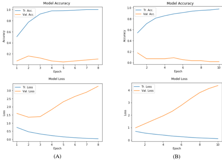
Figure 35: Participant 7958 (A) TCN Training Curves (B) LSTM Training Curves
