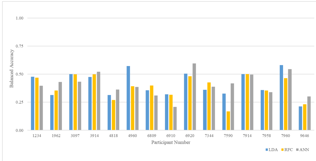
Figure 41: Frequency Features per Task Model Balanced Accuracy
