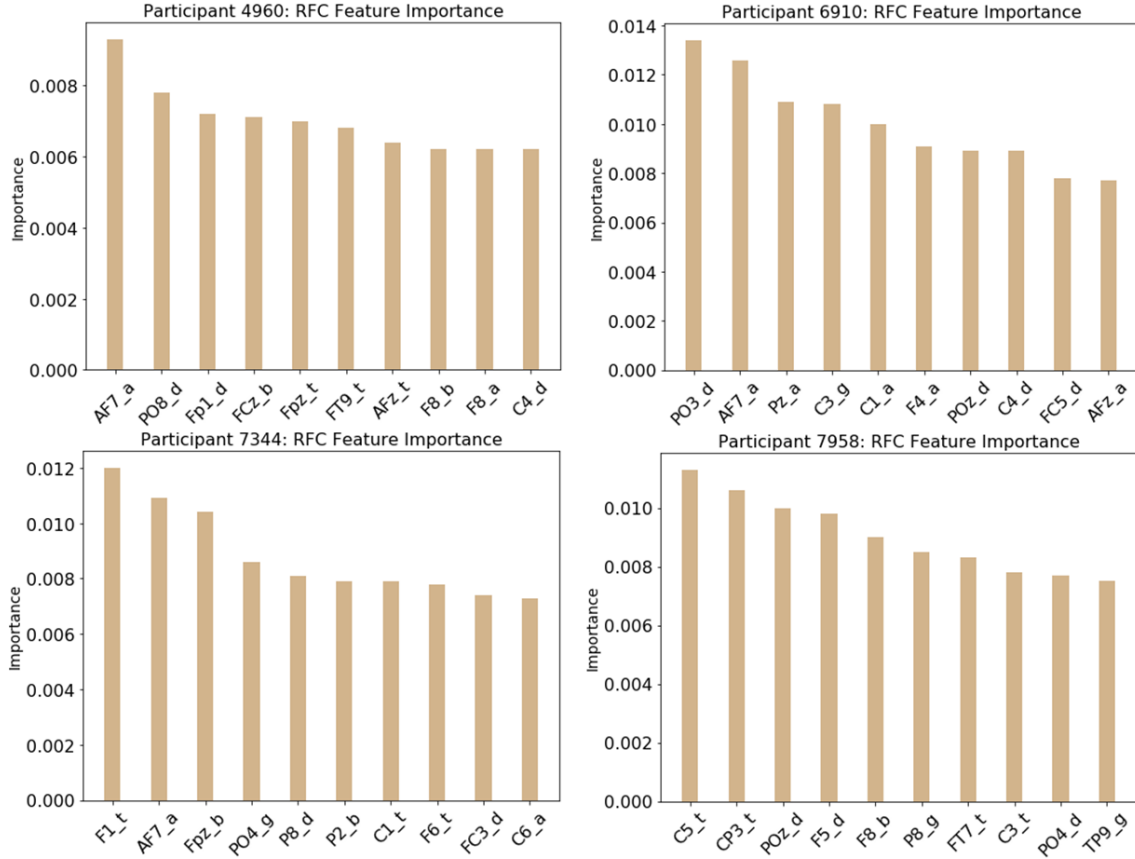
Figure 57: Top Ten RFC Salient Features
