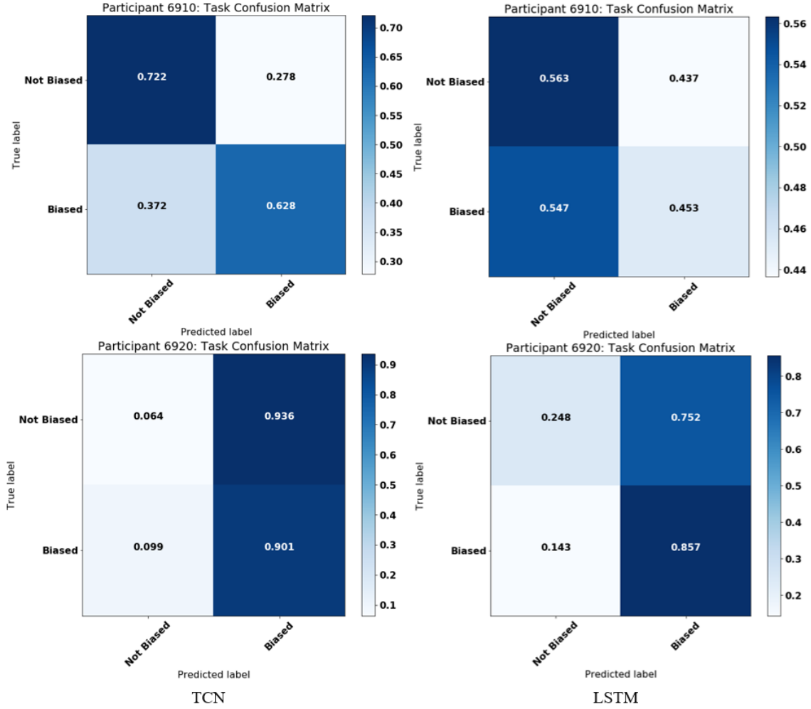
Figure 39: Confusion Matrices of (Left) TCN, (Right) LSTM
