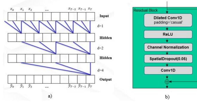
Figure 1: TCN architecture (a) Dilated causal convolutions (b) Residual block
