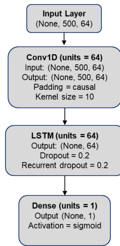
Figure 24: LSTM architecture diagram
