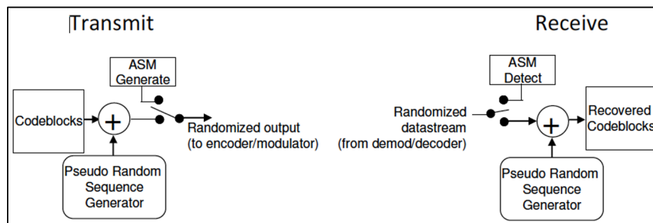
Figure 27-8. Pseudo-Randomization Block Diagram
