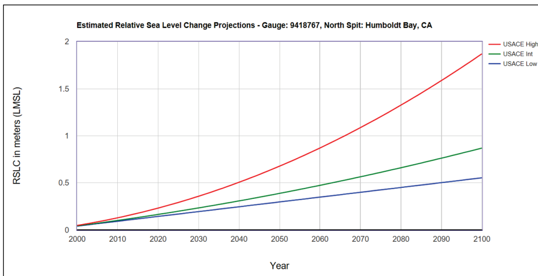
Figure 3. Projected low, intermediate, and high SLR curves at North Spit: Humboldt, California, from 2000 to 2100.
