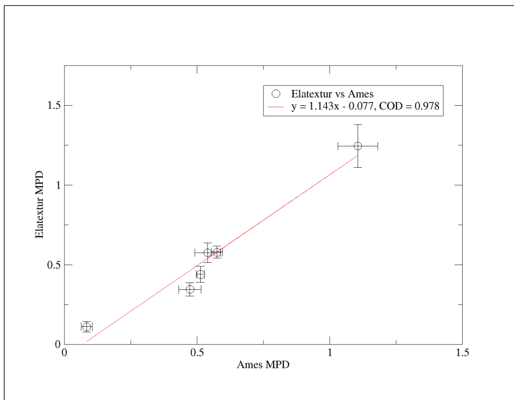
b) Elatexur vs. Ames regression
