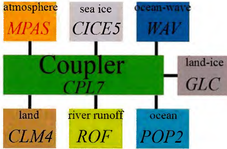
FIG. 10. MPAS-CESM is a fully-coupled Earth system model with a high-resolution nonhydrostatic atmospheric component. Configuration of the MPAS-CESM. This fully coupled Earth System prediction system consists of seven geophysical models: atmosphere (MPAS-A nonhydrostatic), sea-ice (CICE5), land (CLM4), river-runoff (ROF), ocean (POP2), land-ice (GLC), and ocean-wave (WAV). A coupler (CPL7) coordinates the geophysics models time evolution and passes information between them.
