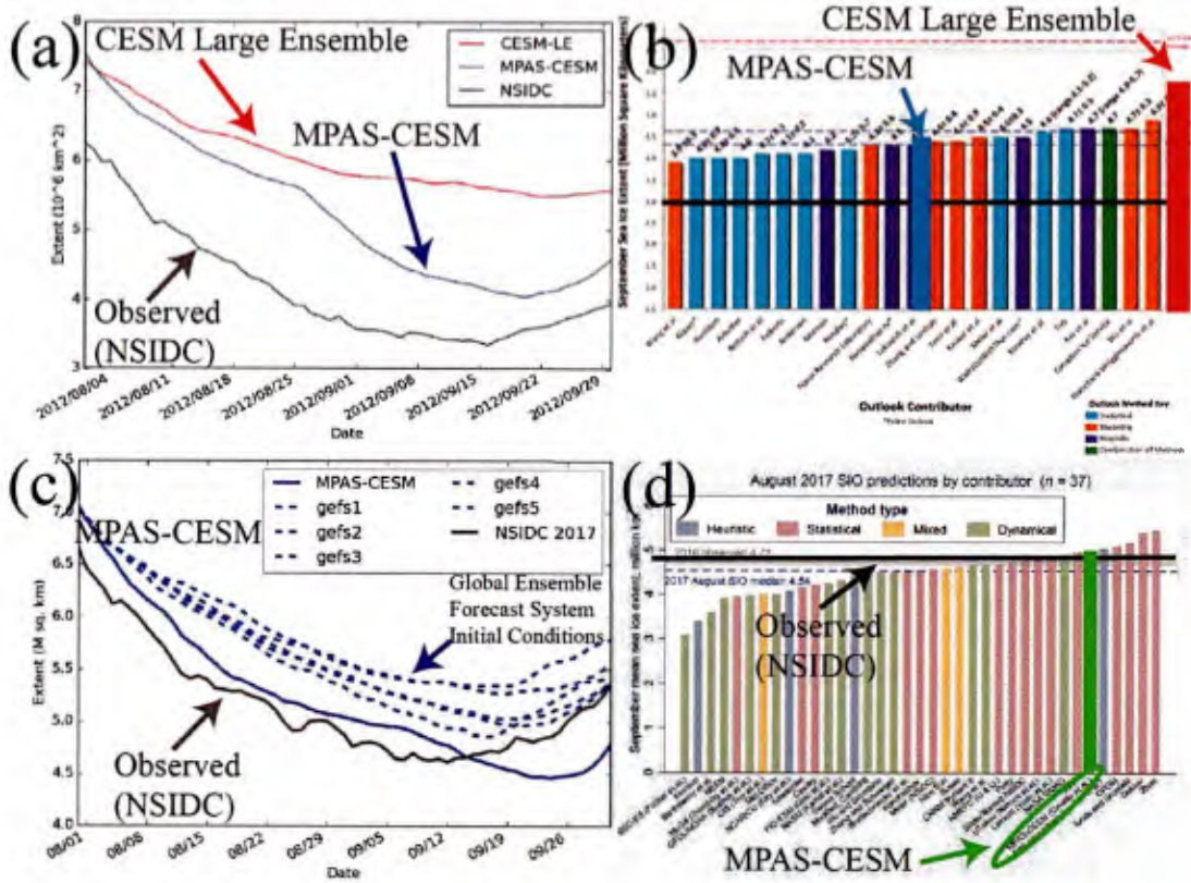
FIG. 12. MPAS-CESM produces competitive subseasonal-to-seasonal forecasts of September minimum sea ice extent. MPAS-CESM Study of Environmental Arctic Change (SEARCH) Sea Ice Outlook (SIO) forecasts of September Arctic sea ice extent initialized 1 August (a)-(b) 2012 and (c)-(d) 2017 with a (a),(c) time series of sea ice extent (SIE) and (b),(d) ranking of mean September SIE in comparison to all other SEARCH SIO forecasts.
