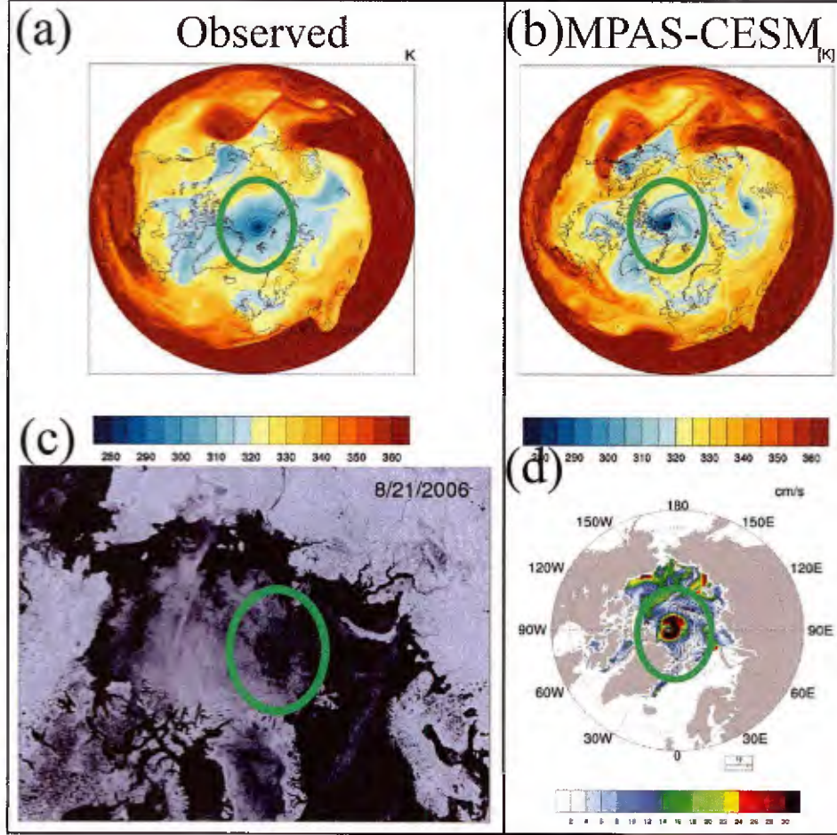
FIG. 5. (a),(c) Observations vs. (b),(d) numerical modeling simulation of a hole in Arctic sea ice underneath an Arctic cyclone and tropopause polar vortex. (a)-(b) Potential temperature on the dynamic tropopause (colors; color interval 5 K) and sea level pressure (black contours; contour interval 4 hPa; only values at or below 1004 hPa are shown) 00 UTC 21 August 2006, (c) sea ice concentration from passive microwave satellite radiometry composited over 21 August 2006, and (d) modeled sea ice velocity ( \text{cm s}^{-1} ). The green circle highlights a region of sea ice loss, evident by satellite observations (c) under an observationally-based model analysis of a TPV and Arctic cyclone in (a). The dynamic tropopause is the 2 PVU surface, where 1 \text{ PVU} = 10^6 \text{ K m}^2 \text{ kg}^{-1} \text{ s}^{-1} . The model simulations in (b) and (d) are from the MPAS-CESM configuration described in this report.
