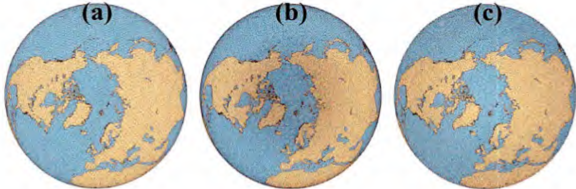
FIG. 2. MPAS is a global model that allows for a smooth grid transition in regions of interest. Schematic of the MPAS C-grid horizontal discretizations that have been implemented for the current study. Comparisons are performed with a (a) uniform mesh containing nearly equal cell spacing globally, (b) and arctic-refined variable resolution mesh where cell spacing varies from \sim 30 -km over the Arctic Ocean to \sim 60 -km in lower latitudes, and (c) a midlatitude-refined variable resolution mesh where cell spacing varies from \sim 30 -km over midlatitude regions and \sim 60 -km over the Arctic region.
