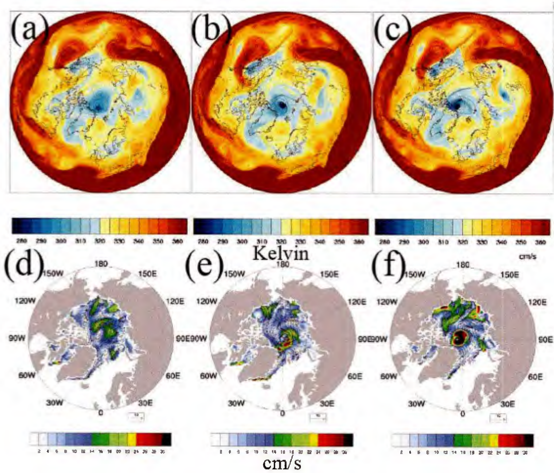
FIG. 14. Stronger TPVs are associated with faster sea ice flow. MPAS-CESM (a)-(c) tropopause potential temperature (colors; units of Kelvin) and sea level pressure (contours; units of hPa; only contoured for values less than 1000 hPa) and (d)-(f) sea ice velocity magnitude (colors; units of \text{cm s}^{-1} ) and motion vectors (arrows) for the (a),(d) X2006, (b),(e) C2006-N50N with -5 K cooling, and (c), (f) C2006-N50N with -10 K cooling simulations at forecast hour 120.
