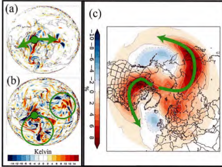
FIG. 9. Bias in TPV intensity spreads upstream and downstream into midlatitudes. MPAS-A (a) 84-h and (b) 144-h forecast differences for an experiment where a TPV was damped during the first 48-h of integration. Forecasts are initialized 4 October 2010 at 00 UTC. (c) ERA-interim (1979-2015) winter TPV track density anomalies (colors) illustrated as the difference between winter and annual TPV probabilities at a given location. Green arrows correspond to the “pathways” of relatively dense TPV tracks in the winter. Green circles in (a) and (b) denote the location where a TPV was damped in the experiment.
