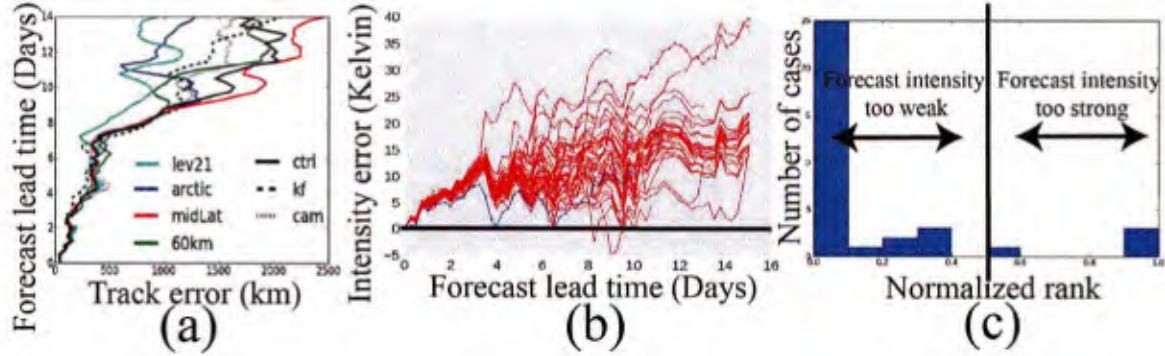
FIG. 7. TPV tracks are predictable for about a week, while intensity forecasts exert an immediate bias. (a) Composite ensemble MPAS TPV track error (x-axis) vs. forecast lead time (y-axis) for the 2006 warm season long-lived TPV. (b) Ensemble TIGGE intensity error (y-axis) vs. forecast lead time (x-axis) for the 2007 warm season long-lived TPV. (c) Rank histogram of TPV intensity in the TIGGE ensemble. Error is the difference between the forecasts and ERA-interim reanalysis values (Forecast minus reanalysis). (c) Rank histogram of TPV 5-d intensity error in TIGGE for all TPVs that are intensifying at analysis time for the time period October 2006 - June 2015. In (b), intensity is defined as the minimum potential temperature on the 2-PVU dynamic tropopause in the vortex. Thus positive (negative) values in (b) imply the forecast vortex is weaker (stronger) than the estimate from reanalysis data. The blue line in (b) represents the ensemble member with the highest resolution. In (c), a lower (higher) normalized rank corresponds to an ensemble member with a forecast vortex that is weaker (stronger) than the estimate from reanalysis data.
