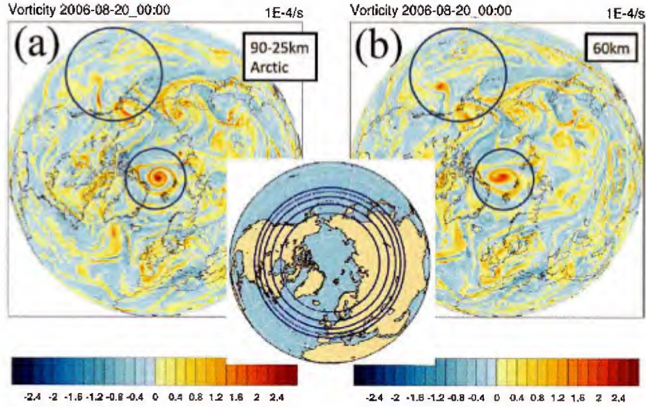
FIG. 11. The mesoscale structure within TPVs becomes apparent with higher atmospheric resolution. 500 hPa relative vorticity at forecast hour 120 from MPAS-CESM with (a) variable resolution with 25-km mesh spacing over the Arctic that smoothly transitions to 90-km spacing elsewhere, and (b) MPAS-CESM globally uniform 60-km mesh spacing. Forecasts are initialized 00 UTC 15 August 2006 from ERA-interim initial conditions.
