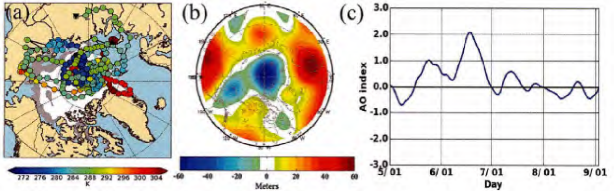
FIG. 6. The negative 500 hPa height anomaly over the Arctic and negative AO pattern in the summer season of 2006 are associated with a single, long-lived TPV. (a) Vortex tracks with vortex intensity (colors) of a unique TPV during June-August 2006 from ERA-interim analyses (Dee et al. 2011). (b) Mean 2006 June-August 500 hPa geopotential height anomalies from NCEP/NCAR Reanalyses (Kalnay and collaborators 1996). (c) 10-d running mean of the Arctic Oscillation (AO) index from May - September 2006 (Data source: NOAA Climate Prediction Center).
