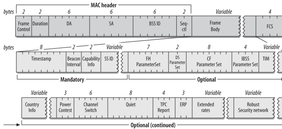
Figure 1. Beacon frame structure. Source: [8].
