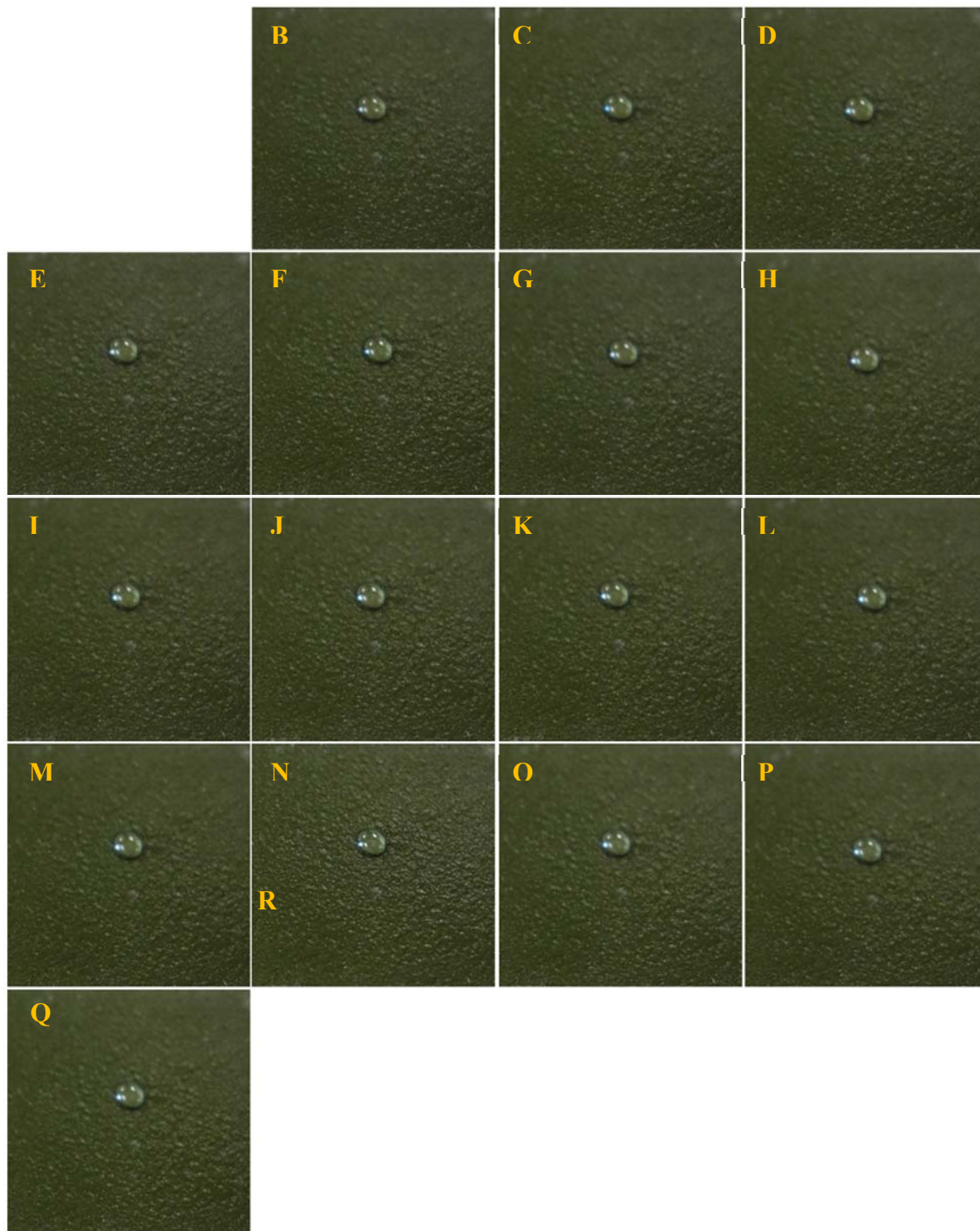
Fig. C2 — MES on Coating #1. Images of a coupon at 0 (B), 0.5 (C), 1 (D), 1.5 (E), 2 (F), 2.5 (G), 3 (H), 3.5 (I), 4 (J), 4.5 (K), 5 (L), 10 (M), 15 (N), 20 (O), 25 (P), and 30 (Q) min following application of the target.
