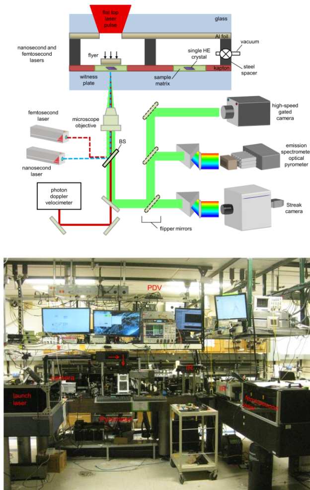
Fig. 26. Shock compression microscope.
