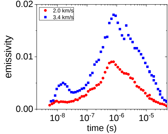
Fig. 37. Time-dependent emissivities of XTX-8003 with 2.0 km/s and 3.4 km/s shocks in the slower and faster cooling regimes, respectively. The emissivities are proportional to the hot spot density.
