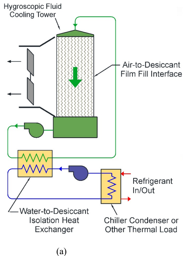
Figure 1. a) Simplified integration schematic of the hygroscopic cooling tower technology and b) example image of an SPX Cooling Technologies (SPX) Marley Aquatower®, a conventional wet cooling system that will be converted to hygroscopic cooling operation for the ESTCP demonstrations.
