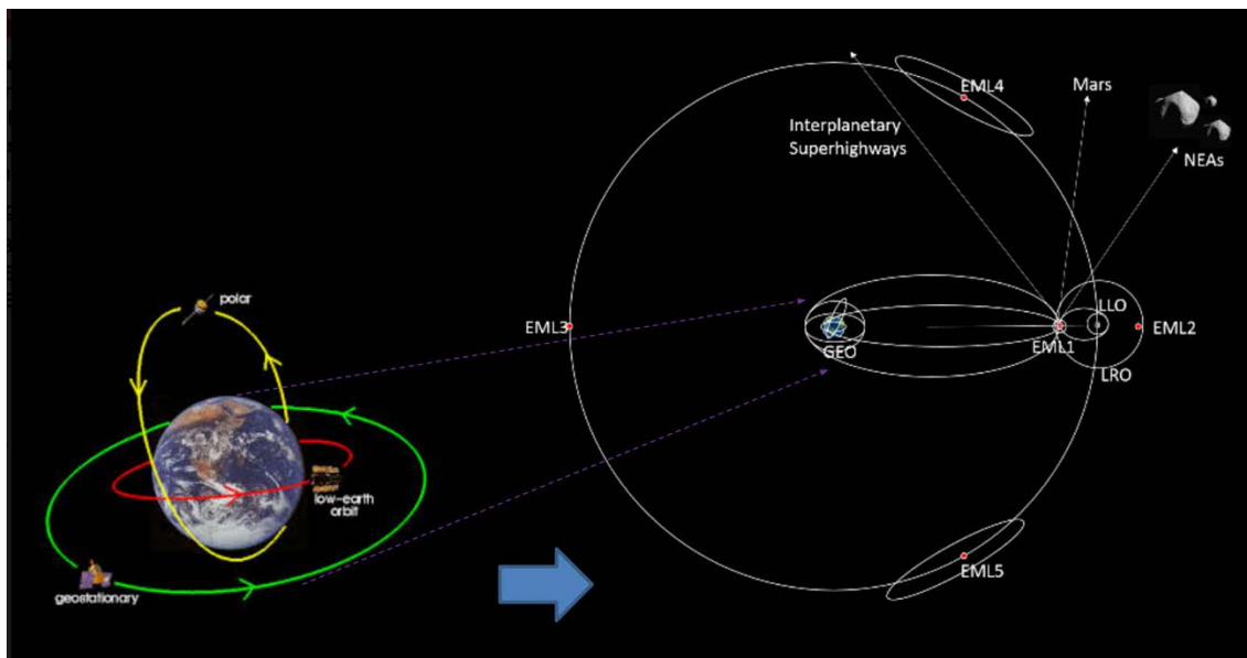
Figure 5.4. A Geo-Centric vs Cis-Lunar View
