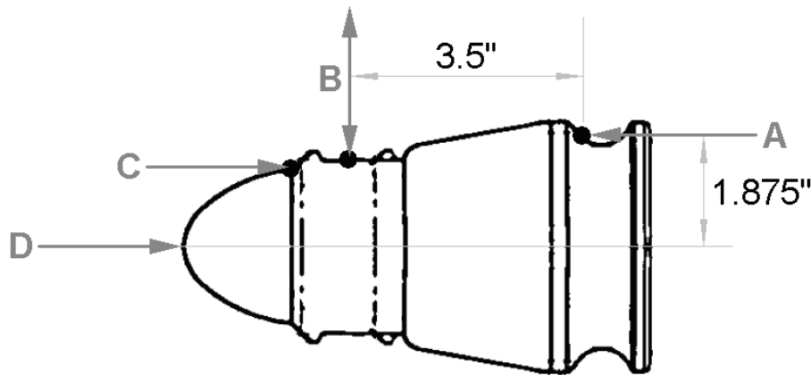
Figure 1: Probe Load Application Locations
