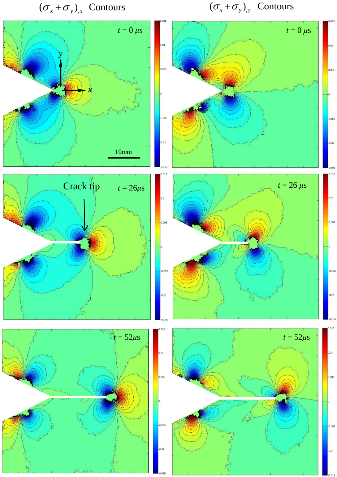
Figure 2. Mode-I stress gradients (contour interval = 1 \times 10^{-3} rad) of (\sigma_x + \sigma_y) in the x- and y-directions for a polycarbonate recorded at 500,000 fps. ( t = 0 corresponds to crack initiation)
