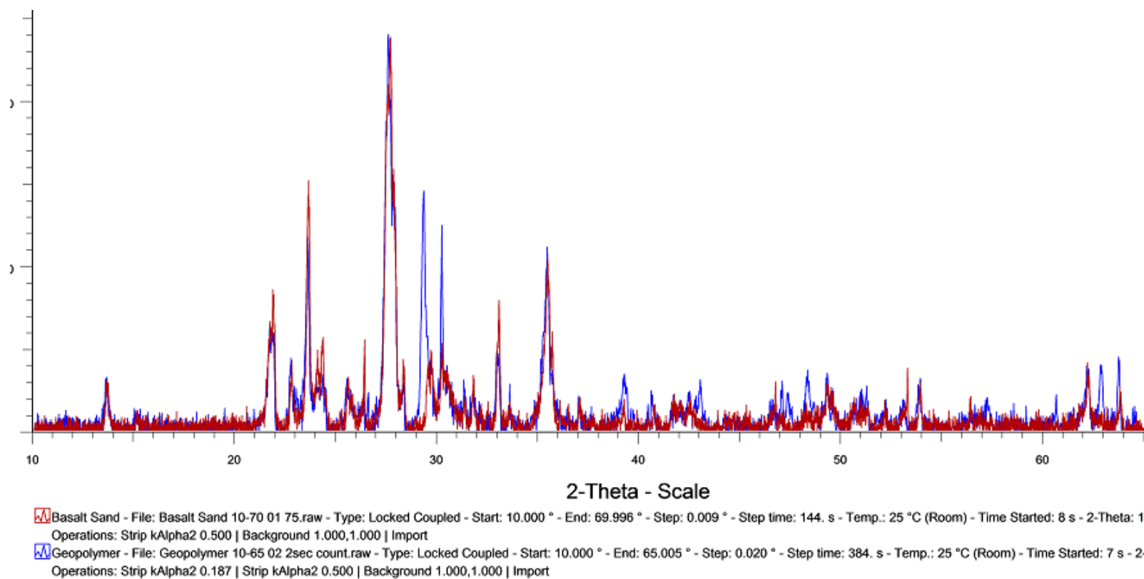
Figure 55. XRD image of geopolymer overlaid with XRD image of basalt sand
