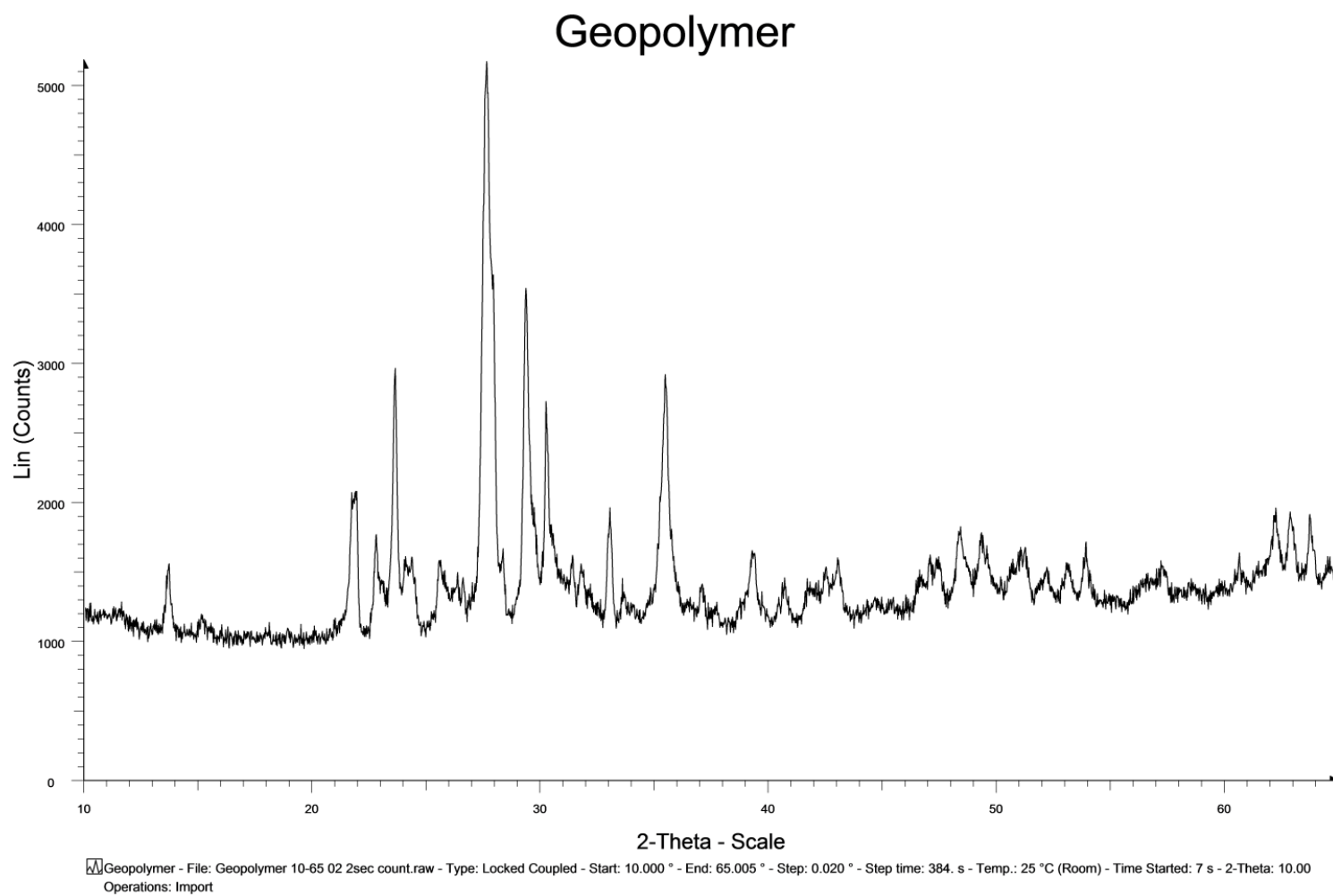
Figure 53. Raw XRD image of geopolymer
