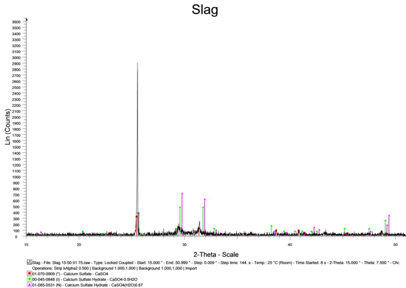
Figure 31. Smoothed XRD image of slag with calcium sulfate, calcium sulfate hydrate, and calcium sulfate hydrate mineralogical identifications
