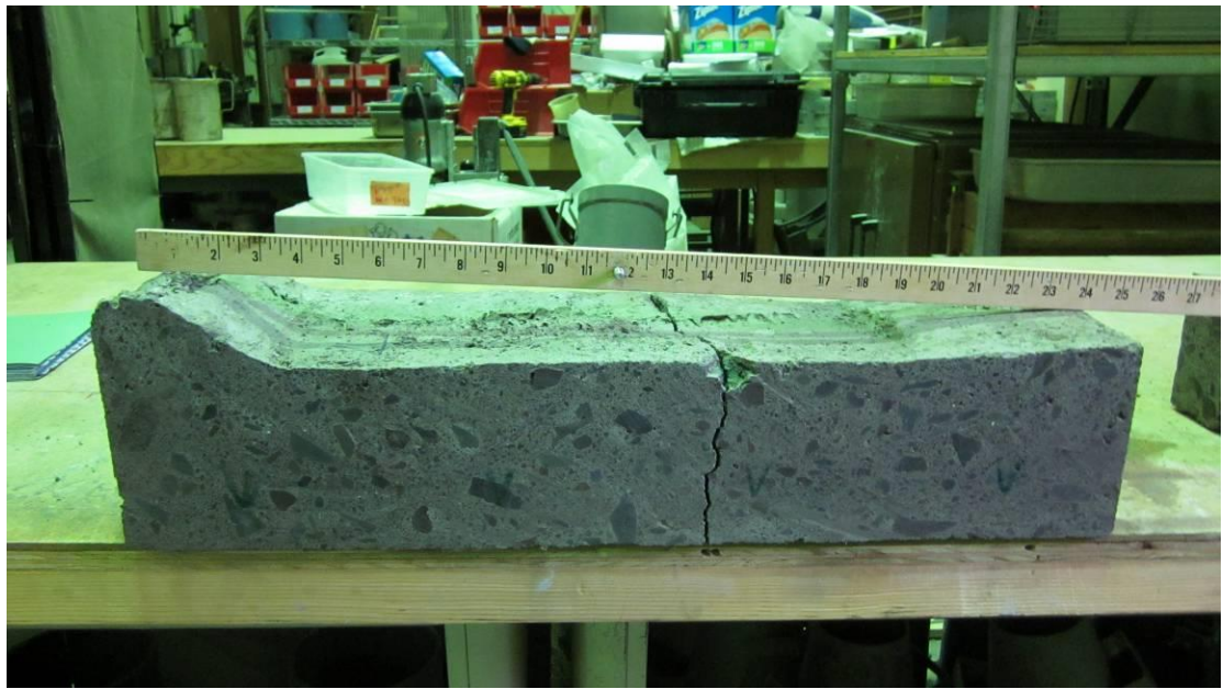
Figure 60. Beam 4
