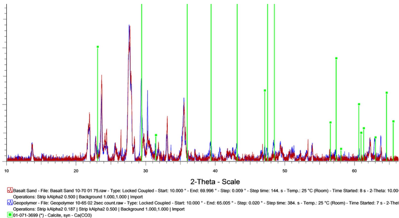
Figure 56. XRD images of geopolymer and basalt sand overlaid with calcite mineralogical identification
