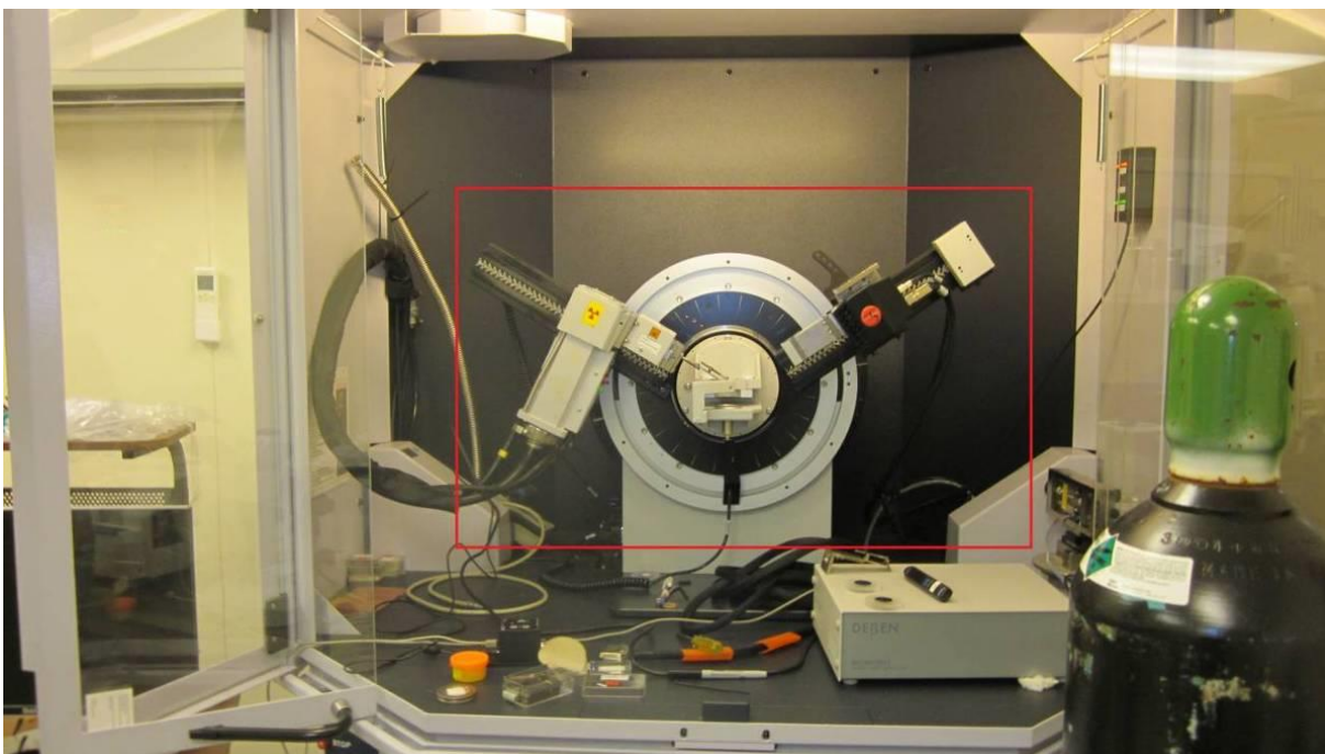
Figure 25. Bruker-Nonius Kappa CCD X-ray Diffractometer; red box highlights the goniometer.
