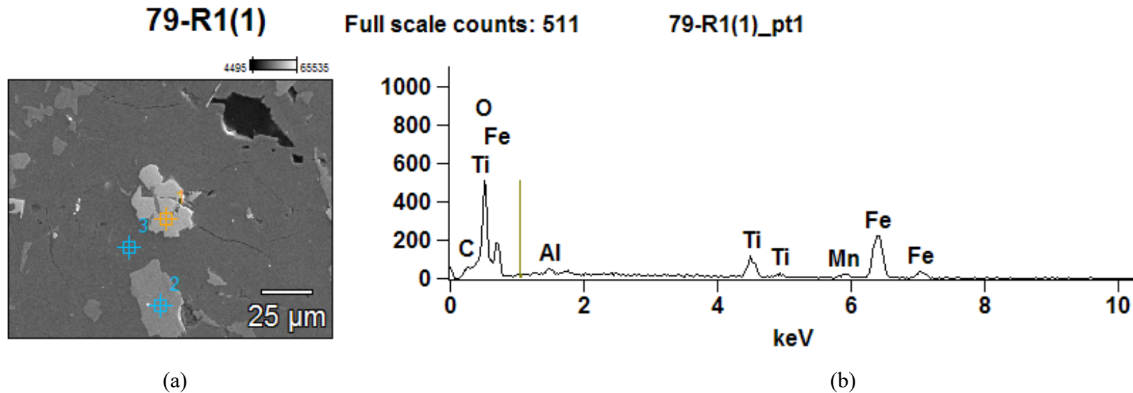
Figure 40. (a) Backscatter electron image of basalt in the geopolymer (b) elemental composition of point 1 consisting predominantly of oxygen, titanium and iron suggesting and ulvöspinel.
