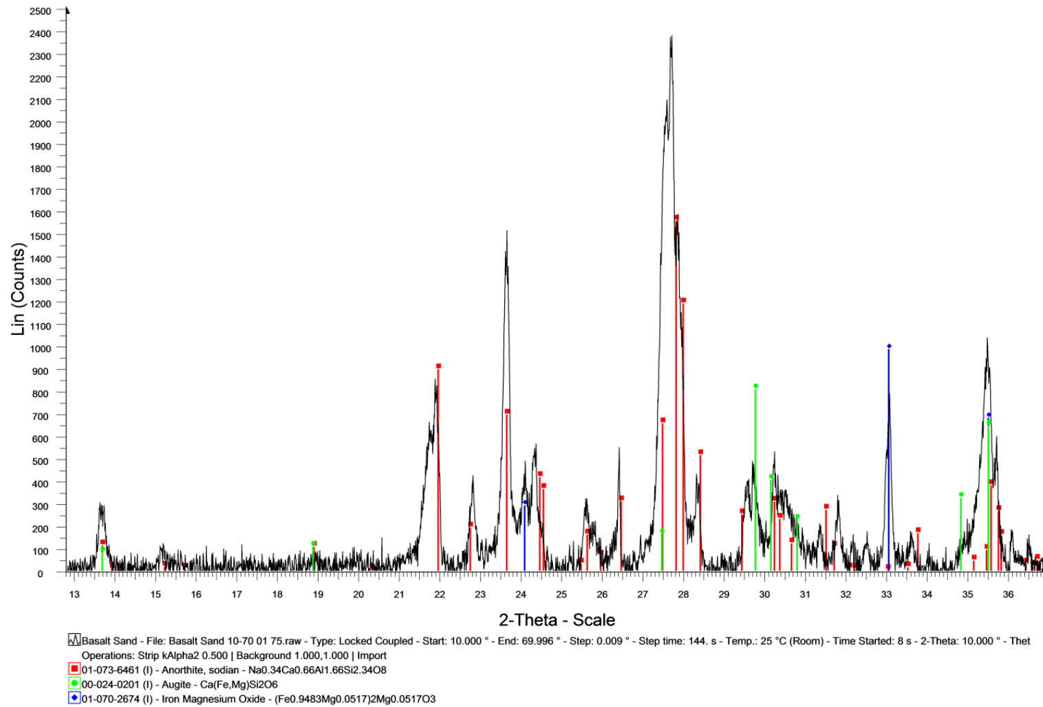
Figure 38. Smoothed XRD image of basalt sand with mineralogical identification
