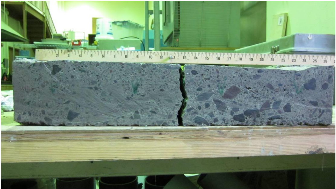
Figure 62. Beam 6
