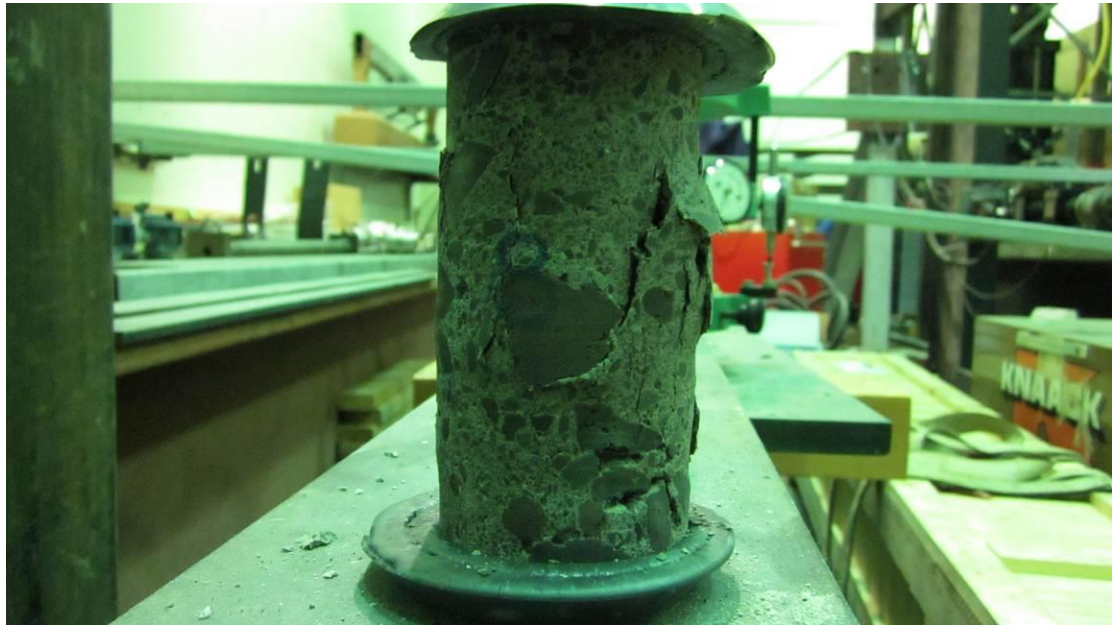
Figure 72. 2.25-inch-diameter Cylinder 8
