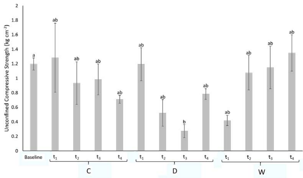
Figure 9. Unconfined compressive strength measurements. Each bar is an average of three replicates; error bars indicate standard error. Letters of significance indicate values that are significantly different from one another ( p = 0.0062 ).
