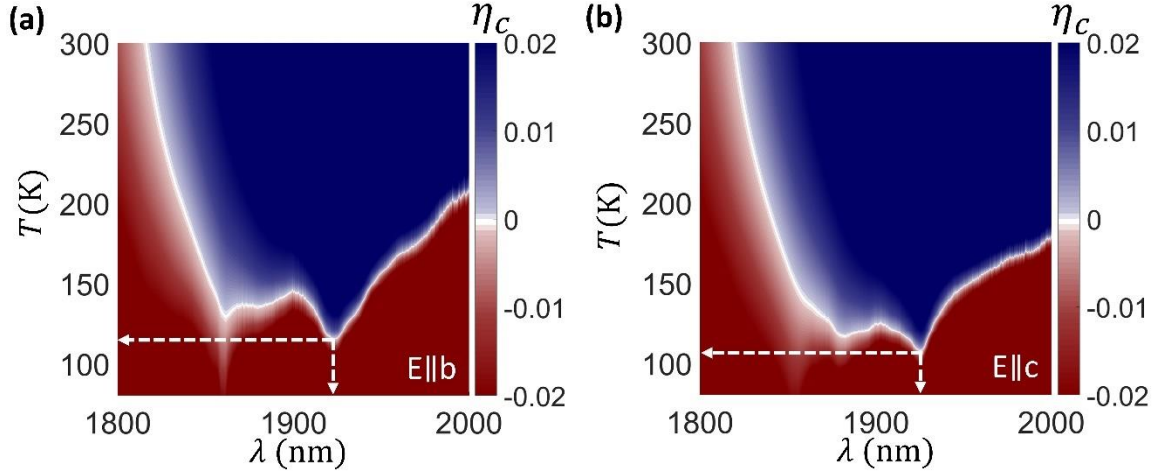
Figure A23: Estimated MAT of 1%Tm:BYF with (a) \alpha_b = 2.5e-5 \text{ cm}^{-1} for E \parallel b and (b) \alpha_b = 1.0e-5 \text{ cm}^{-1} for E \parallel c polarizations.
