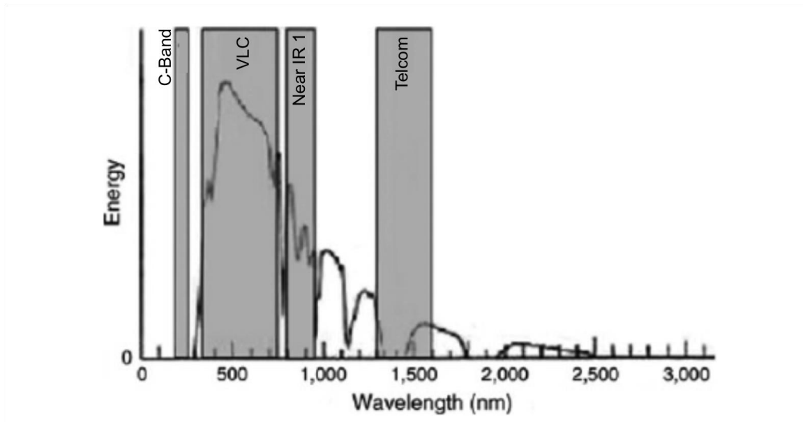
Figure 1. Illustration of the Optical Spectral Bands. Adapted from [1].
