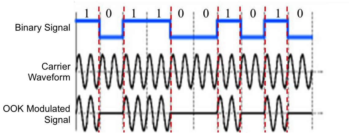
Figure 3. NRZ OOK Modulation Process. Adapted from [3].
