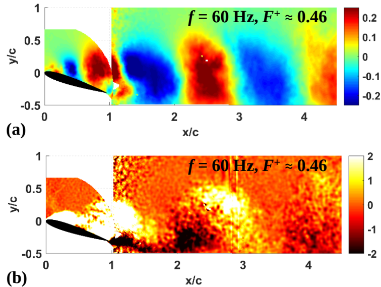
Figure 1. Sample phase-averaged PIV for ns-DBD plasma forcing at F^+ \approx 0.46 ( f_f = 60 Hz) (a) Dimensionless Vertical Fluctuating Velocity (b) Dimensionless Spanwise Vorticity. Re=740,000 ( U=40m/s ) (Ashcraft et al. 2016).
