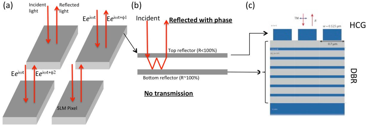
Figure 6 (a) Schematic of GTI spatial light phase modulator (SLPM) composed of one-sided resonators. (b) Due to the asymmetric design of the resonator light just gets reflected with the acquired phase. (c) GTI design with a high reflectivity DBR and a high contrast grating reflector on top.
