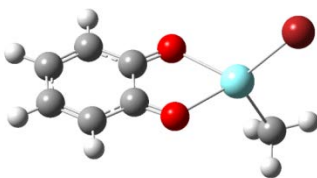
Figure 11 – Predicted MeBr binding to Y catecholate. The Me group and Br atom dissociate and bind separately to the Y atom. The grey atoms are C, the light blue is Y, the bright red are O, and the darker red is Br.
