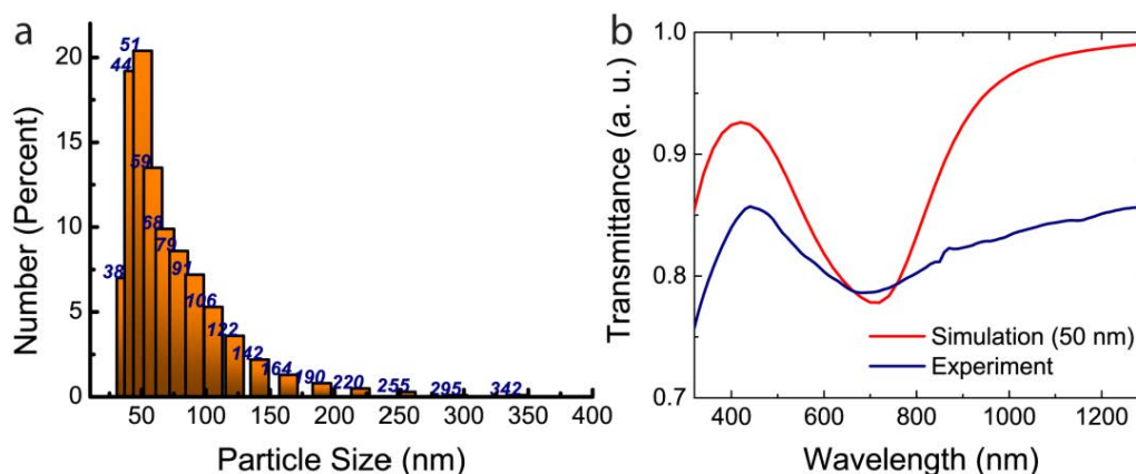
Figure 4: Dynamic light scattering measurement of the size dispersion for colloidal plasmonic TiN nanoparticles. Peak value around 50 nm is a desired size for more efficient cellular uptake. The long tail with marginal large dimensions is likely due to clustering effects. (b) Transmittance data taken from aqueous TiN sample (blue) and calculated data for mono-sized 50 nm nanoparticle solution (red). Calculated transmittance with mono-sized nanoparticle solution agrees well on the peak spectral position and amplitude with the experimental data. Broader experimental peak can be attributed to the size dispersion as observed in dynamic light scattering measurement.
