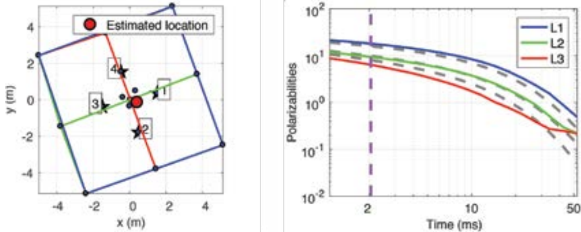
Figure 3. Borehole EM data and analysis for survey shown in Images 5, 6 and, 7. Left: Borehole survey geometry with solid lines indicate transmitters, and numbered stars indicate measured boreholes. The red marker indicates estimated target location; the estimated depth is 3.9 m. Right: Estimated polarizabilities (solid lines) and reference polarizabilities for 500 lb U.S. GP bomb (dashed lines). The vertical dashed line indicates 2 ms time channel for data shown in Figure 4.
