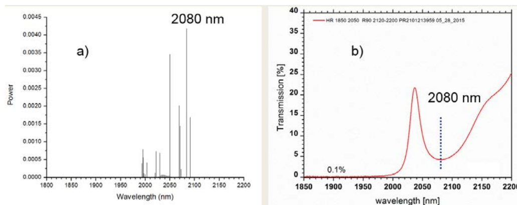
Fig. 6 Demonstration of Tm/Ho fiber lasing a) output spectrum and b) output coupler transmission spectrum
