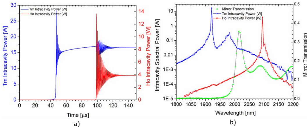
Fig. 13 a) Evolution of the Tm (blue) and Ho (red) laser intracavity power over a 150- \mu\text{s} interval and b) spectral output of the Tm (blue) and Ho (red) laser powers at the end of the 150- \mu\text{s} period. Note the transmission spectra (green) of output coupler used in simulation.
