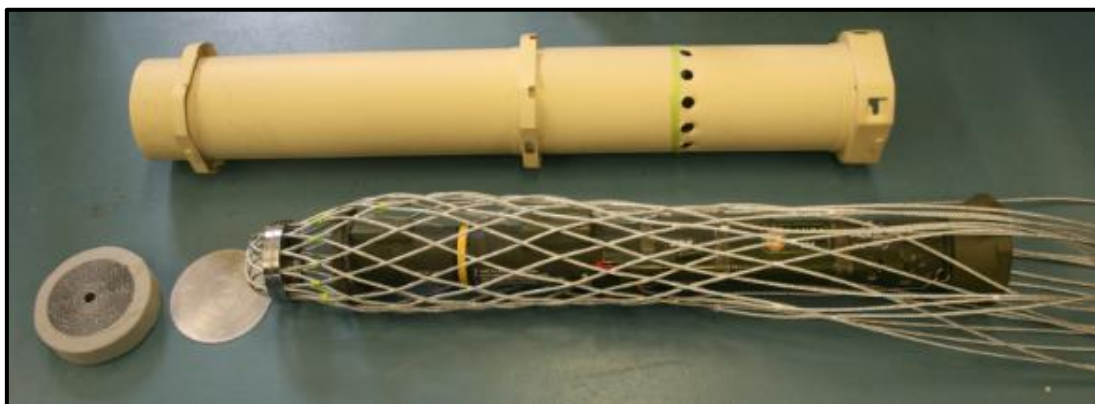
Figure 13 Steel cabled braid around launcher (ruggedized container)
