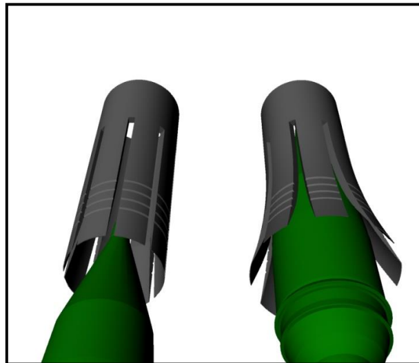
Figure 7 Locking wedge concept
