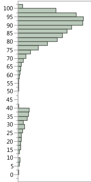
Summary Statistics
