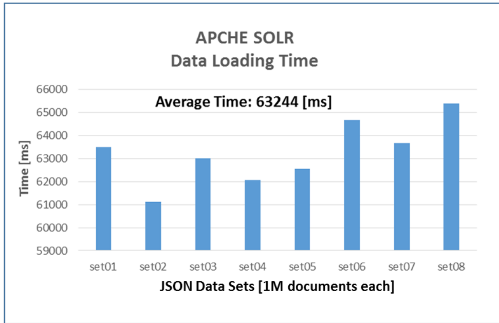
Figure 2-4. Example of Time Required to Load Data Sets into Apache Solr Server
