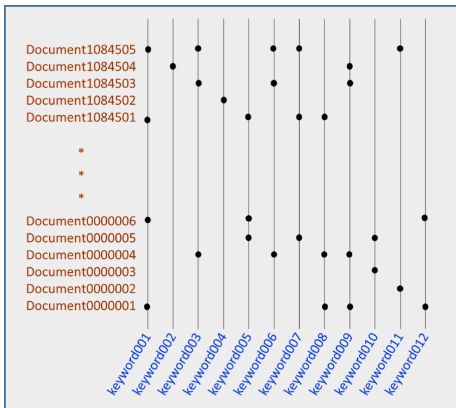
Figure 2-1. Notional Depiction of an Inverted Indexing Approach
