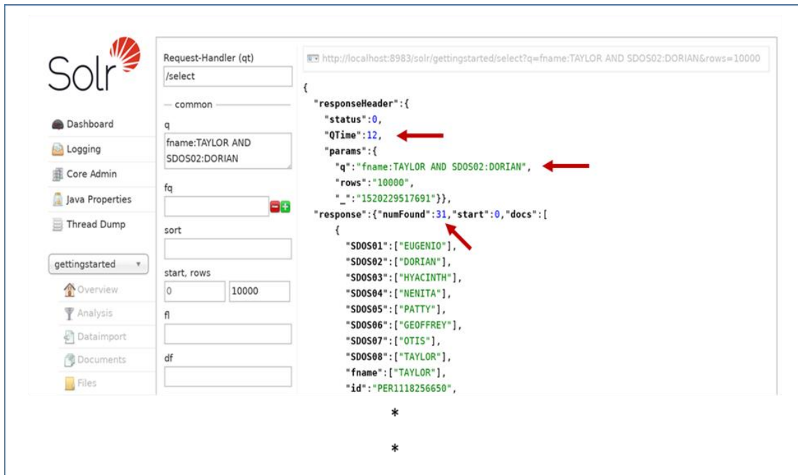
Figure A-3. Results for the SDOS02 Query Using the Solr Admin Interface
