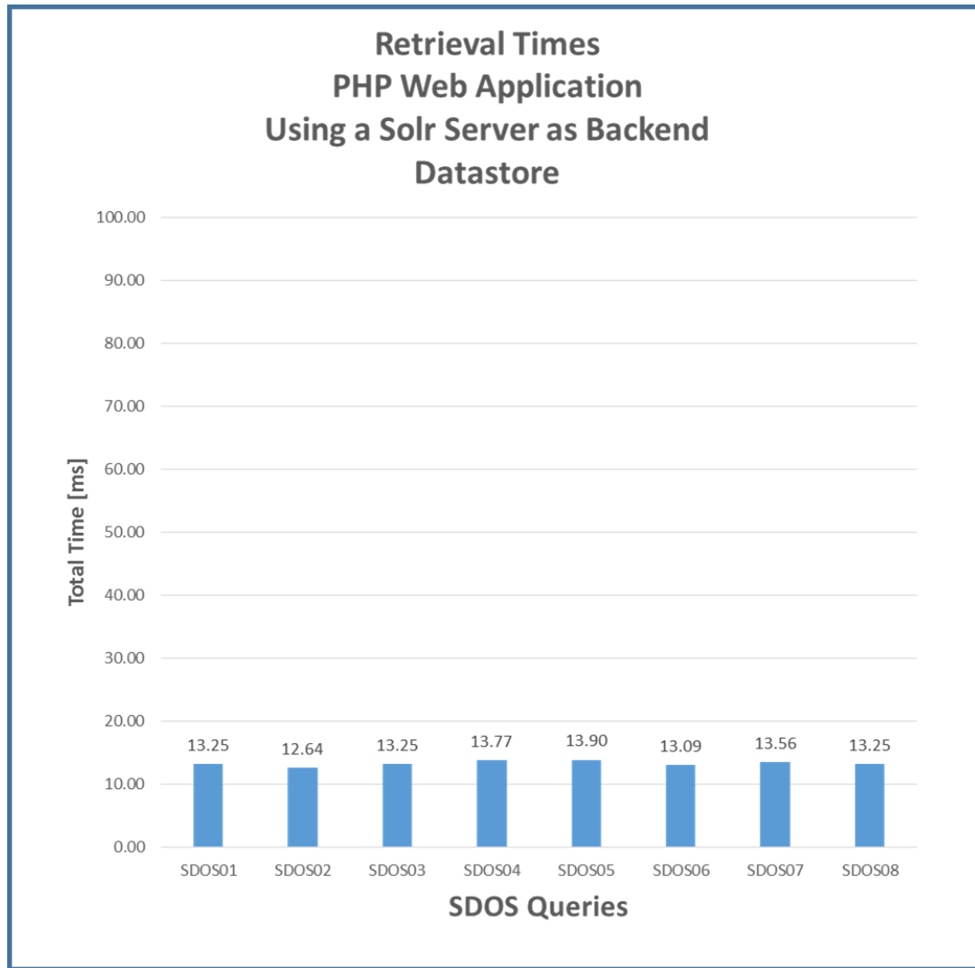
Figure A-9. Data Retrieval Performance for Web Applications Using the Solr Server as Backend Data Store
