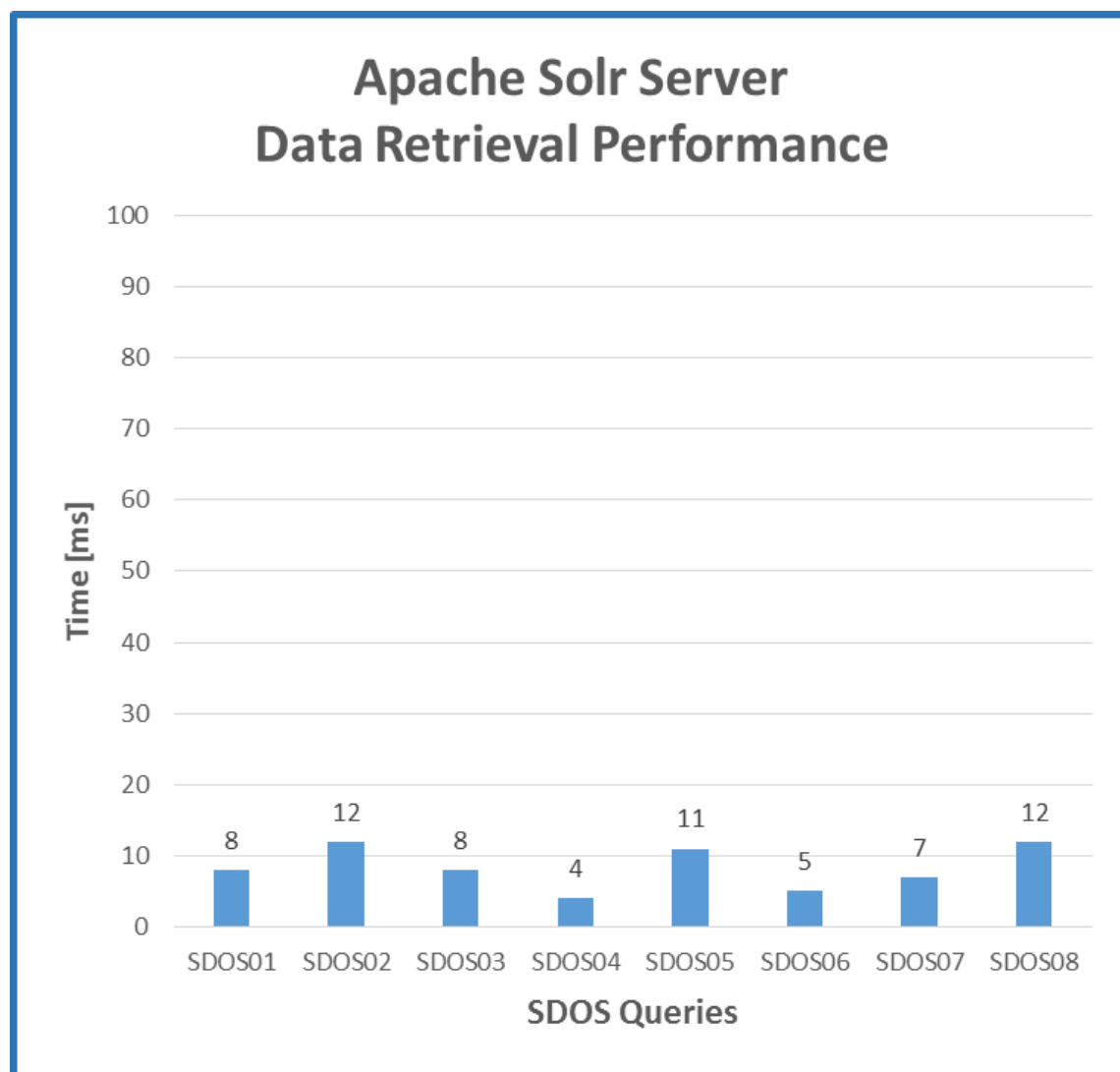
Figure A-5. Apache Solr Server Data Retrieval Times for the SDOS Use Case
