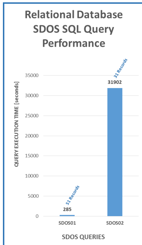
Figure A-7. SQL Query Data Retrieval Times for the SDOS Use Case using 128 Million Entries
