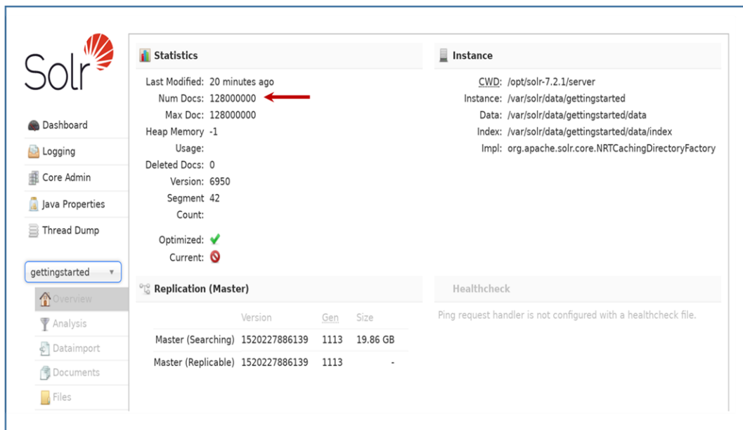
Figure A-1. Screen Capture of the Apache Solr Server Admin Interface with All 128 Million JSON Documents Loaded
