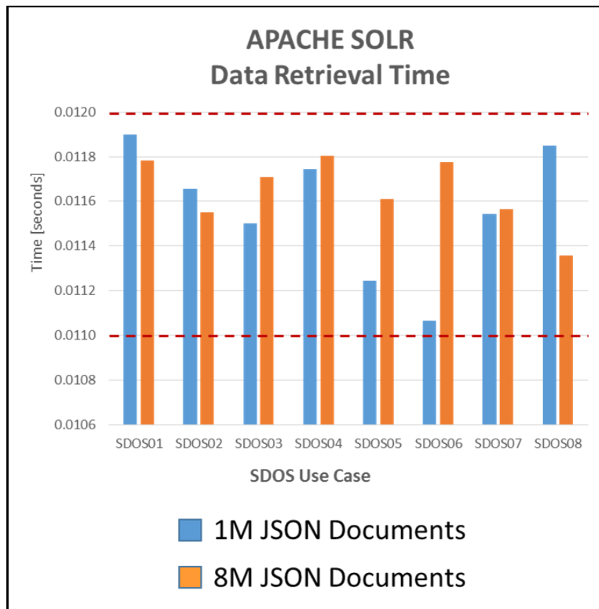
Figure 2-5. Time to Access and Retrieve Data for the “TYLER knows DORIAN” Query
