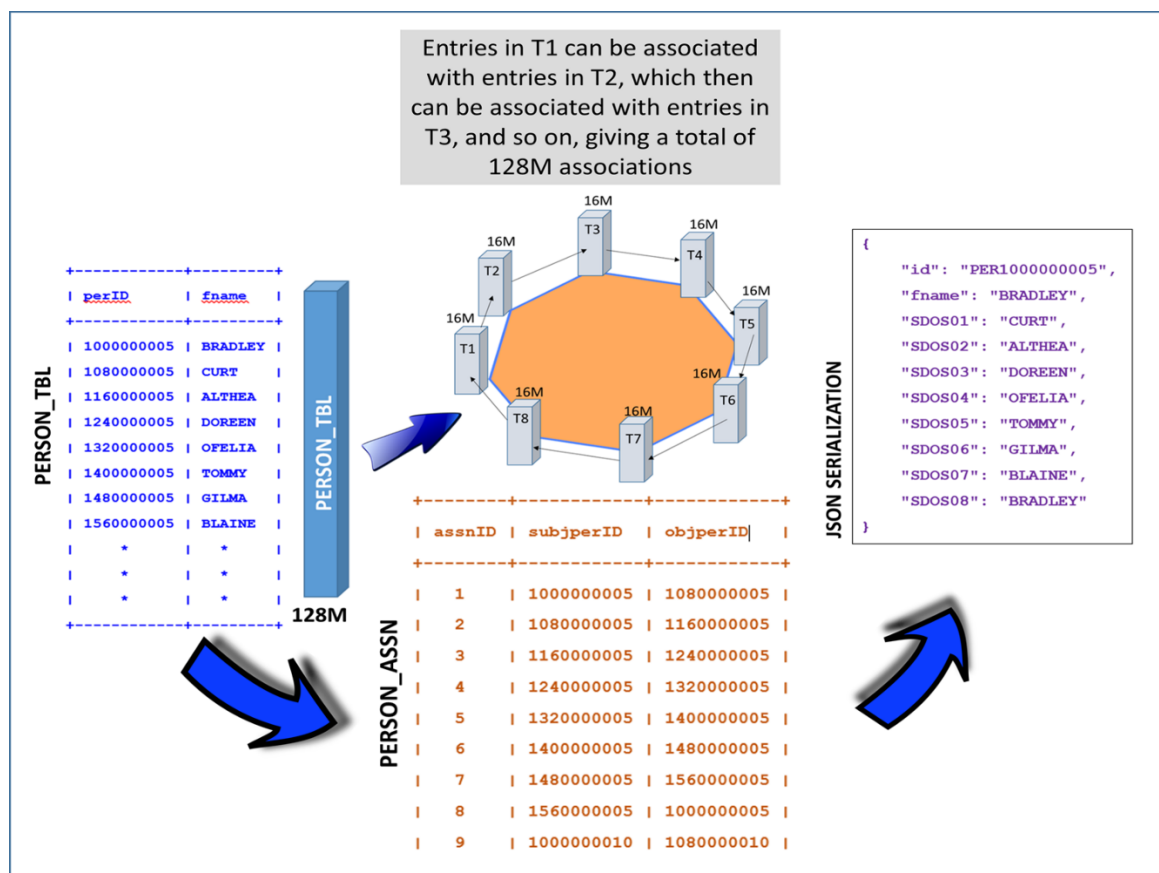
Figure 2-2. Representation of the “Six Degrees of Separation” (SDOS) Use Case as JSON Documents
