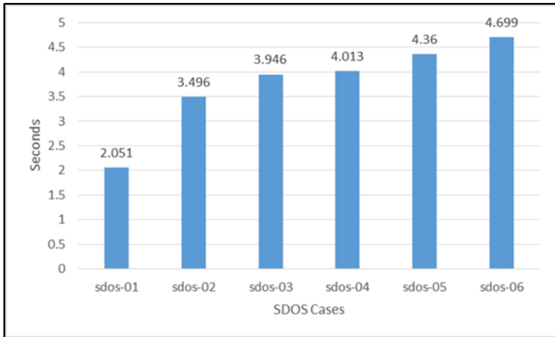
Figure A-6. Prolog Data Retrieval Times for the SDOS Use Case and 8 Million Clauses
