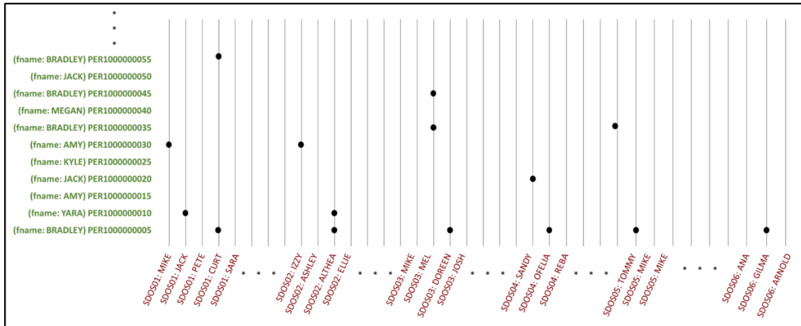
Figure 2-3. Notional Inverted Index Set for the SDOS Use Case
