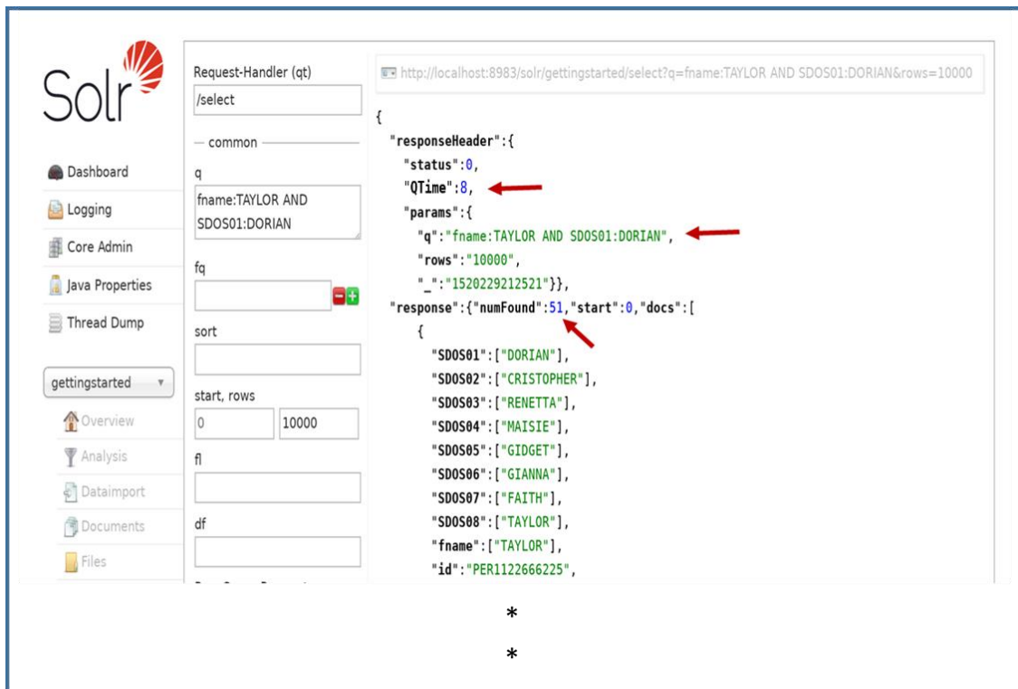
Figure A-2. Results for the SDOS01 Query Using the Solr Admin Interface
