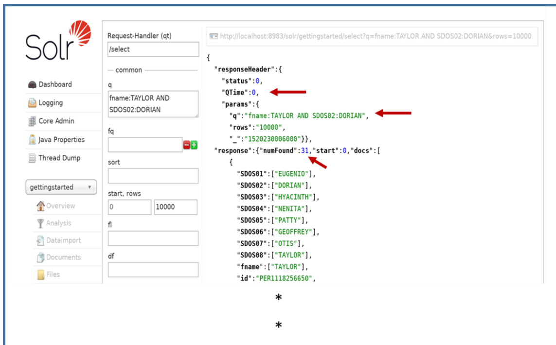
Figure A-4. Retrieval Time for Cached Queries in the Apache Solr Server
