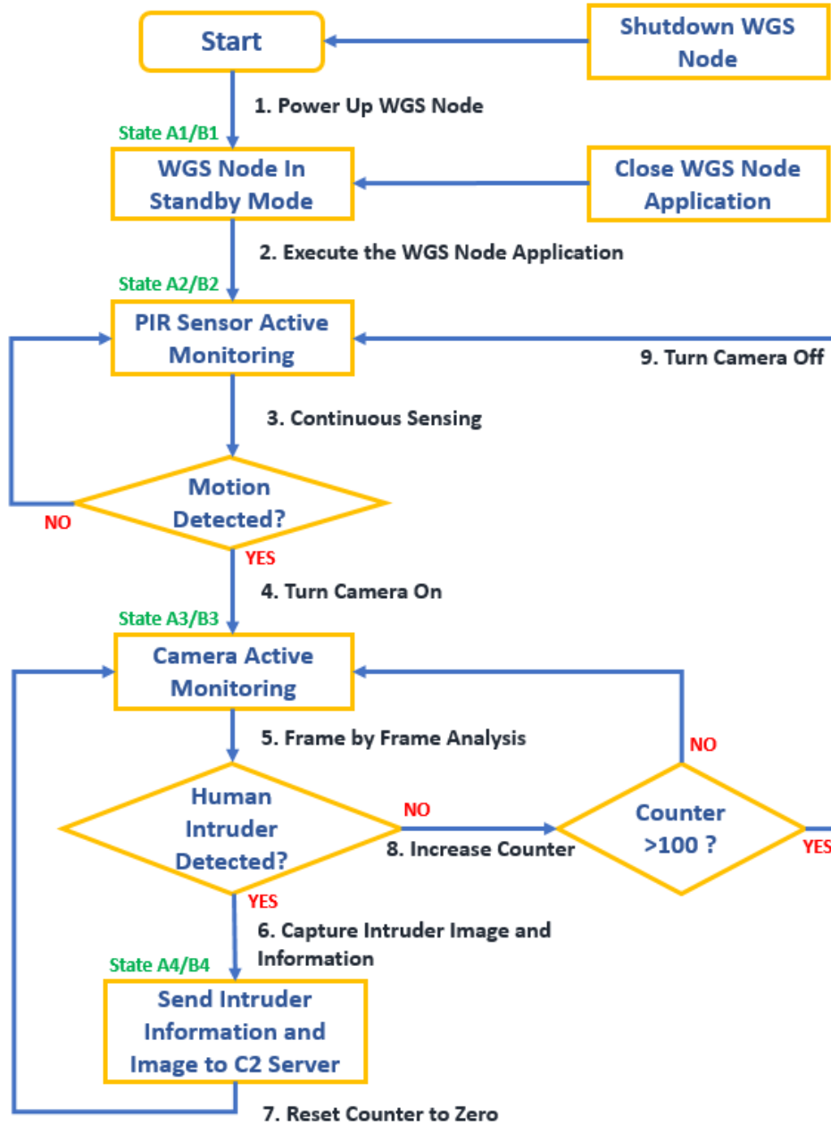
Figure 14. Operating Flow Chart for WGS Node
