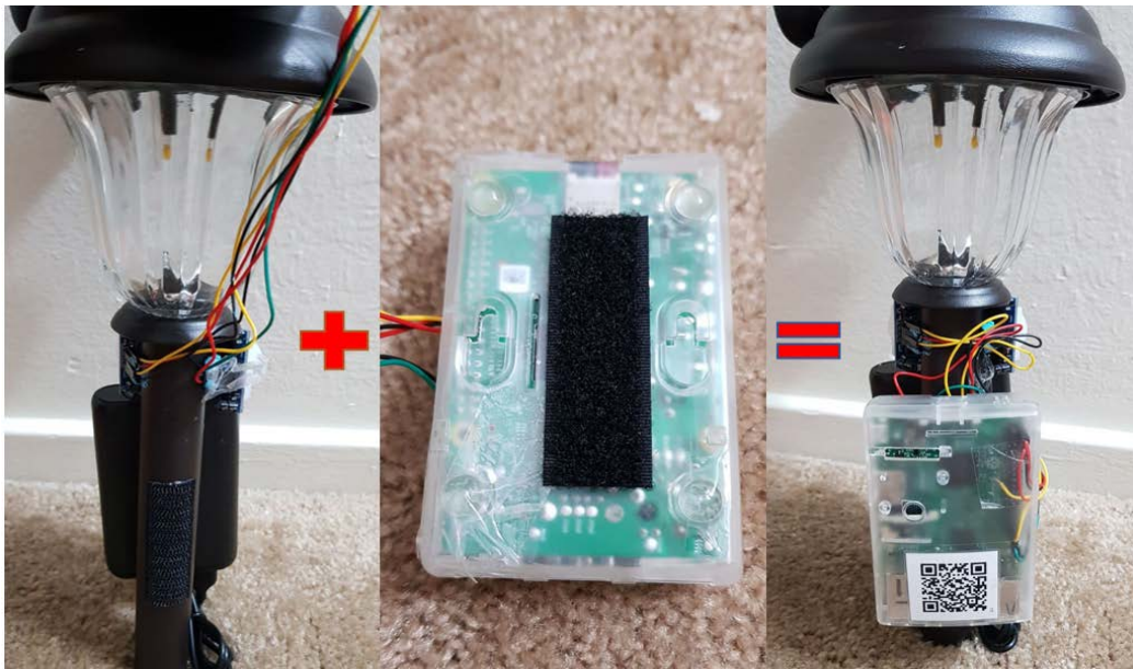
Figure 37. Mounting of Raspberry Pi 3 Model B Board onto the Solar Garden Light for Variant A of WGS Node
