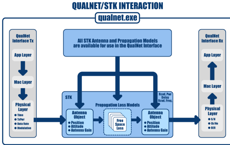
Figure 5. STK/QualNet Interaction. Source: System Tool Kit (2017).
