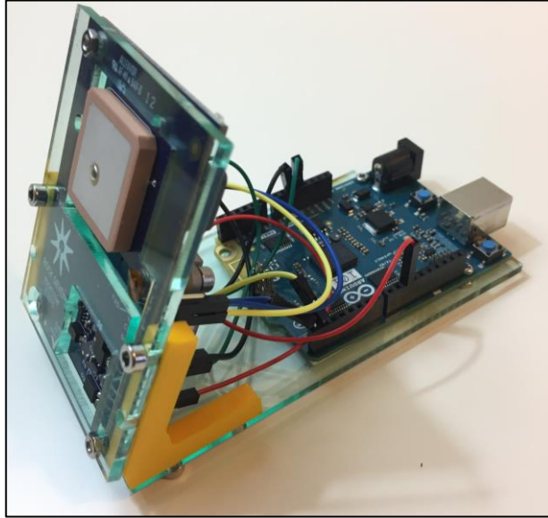
Figure 23. The RockBlock Connected to the Arduino 101
