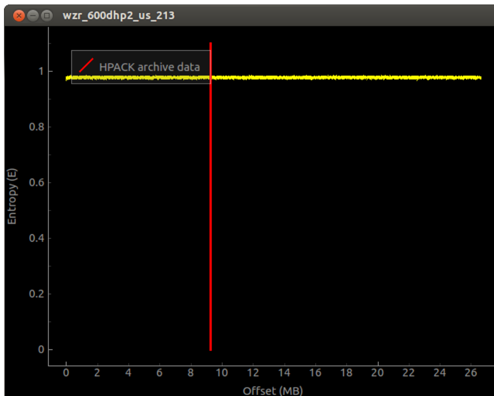
Figure 8: Binwalk Entropy Analysis Graph
