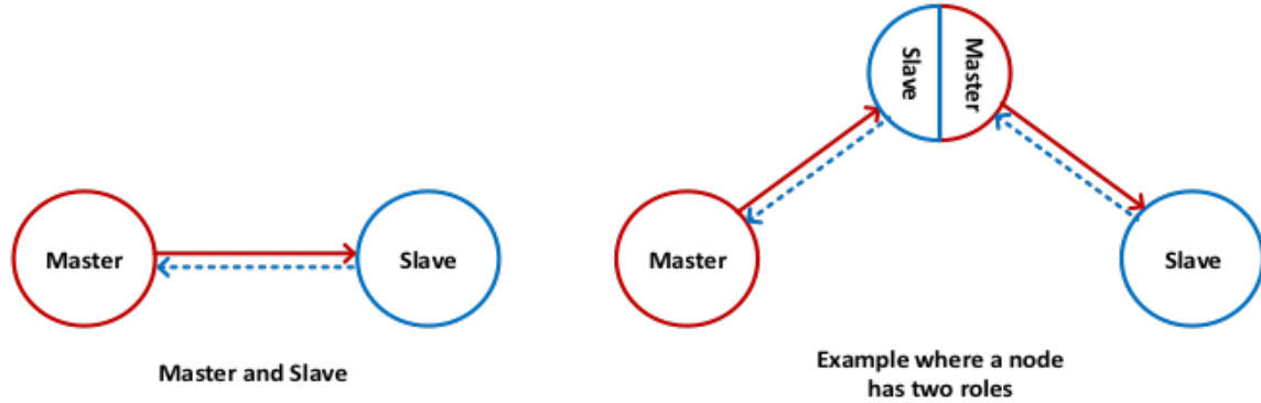
(a) ANT+ Master node sending acknowledged messages to a Slave. (b) An ANT+ Master node pushing acknowledged messages to a Master/Slave node which also pushes acknowledged messages to another Slave node.
