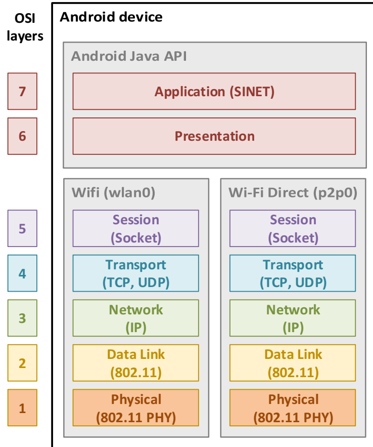
Figure 9. Android Devices Implementing Wifi and Wi-Fi Direct
