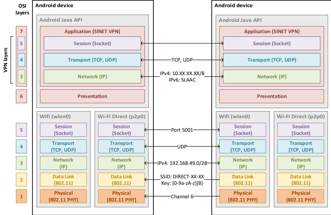
This figure shows how the SINETapp configures the network stack. It builds a VPN which inserts the second set of layers 3–5 within the Application layer. This VPN allows the changes of the mesh to be seamless to the user level Apps.
