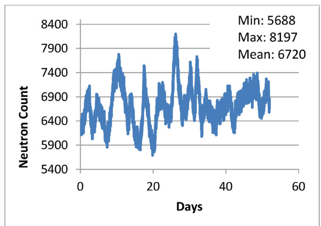
Figure 10. Temporal nature of neutron background: 53 days.
