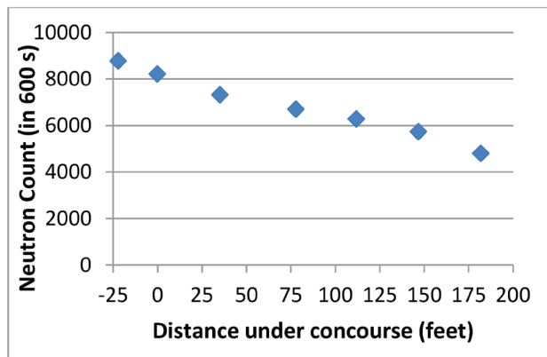
Figure 7. Neutron background on concourse entry showing a 45% reduction in 180 feet.
