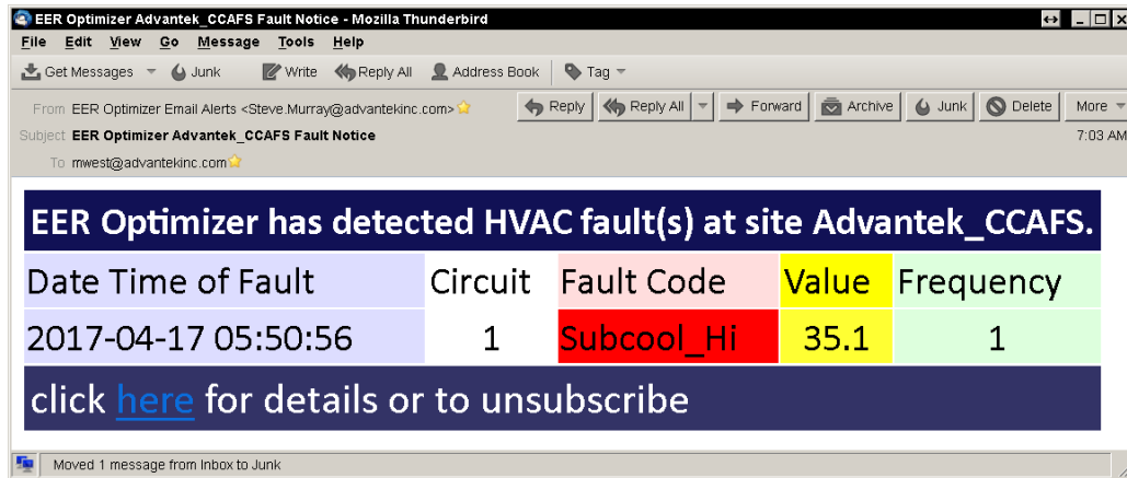
Figure 22. Fault Detection & Diagnostic Email Alert.
