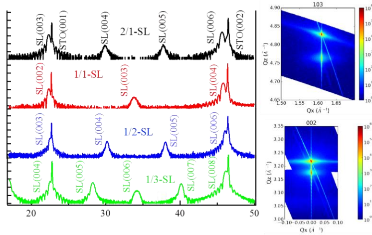
Figure 6. Left: Room temperature \theta - 2\theta scans of the series of nonpolar superlattices (SLs). The corresponding superlattice peaks are also shown. Right: a representative reciprocal spacing mapping of the superlattice at the monolayer limit (1/1-SL) around the (103) and (002) (pseudocubic lattice) film peak.
