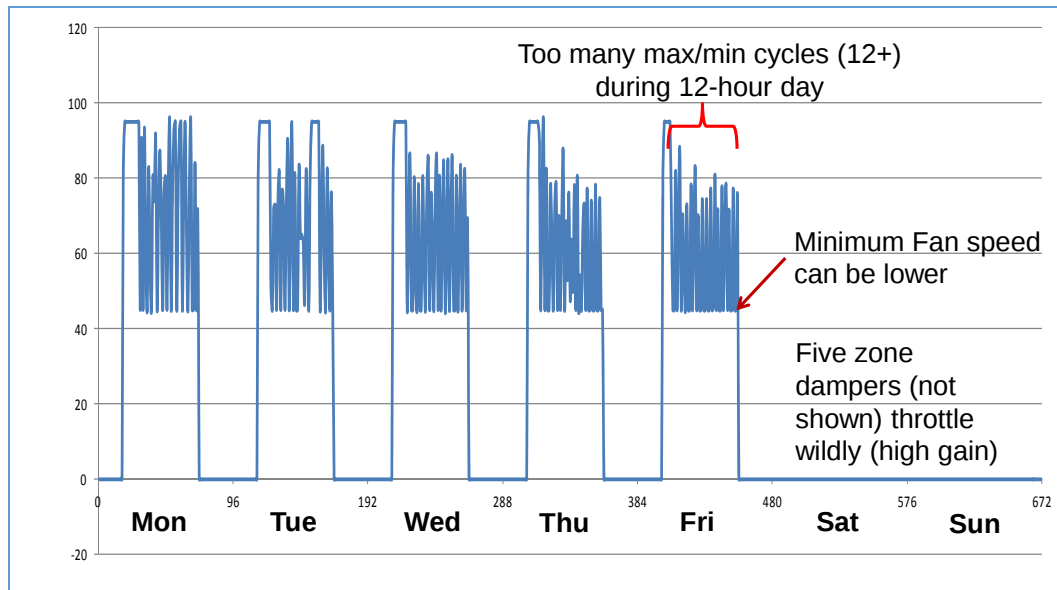
Figure 1. Daily Cycling of AHU-2-001 Supply Fan.
